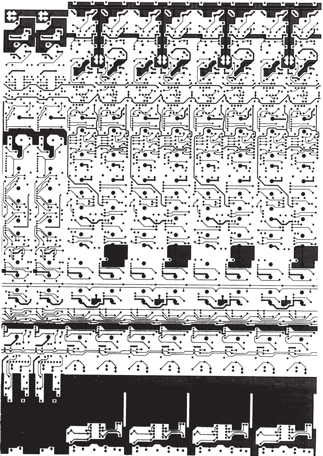
SC3316A ISSUE 3 3-18-94 POWER AMP MIXER MAIN BOARD
