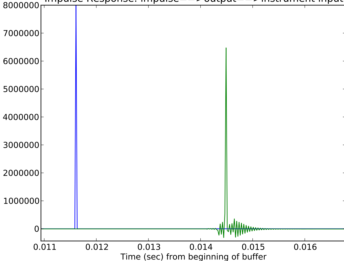
Impulse Response: impulse==>output==>instrument input
