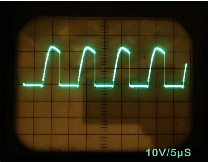
collector of TS47
