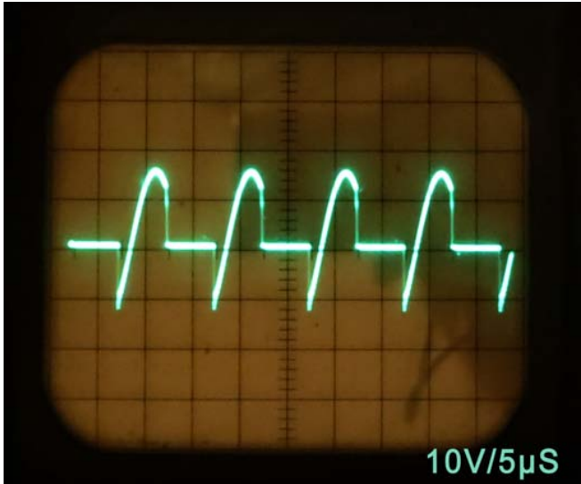
Cathode D53, resonance out of tune
