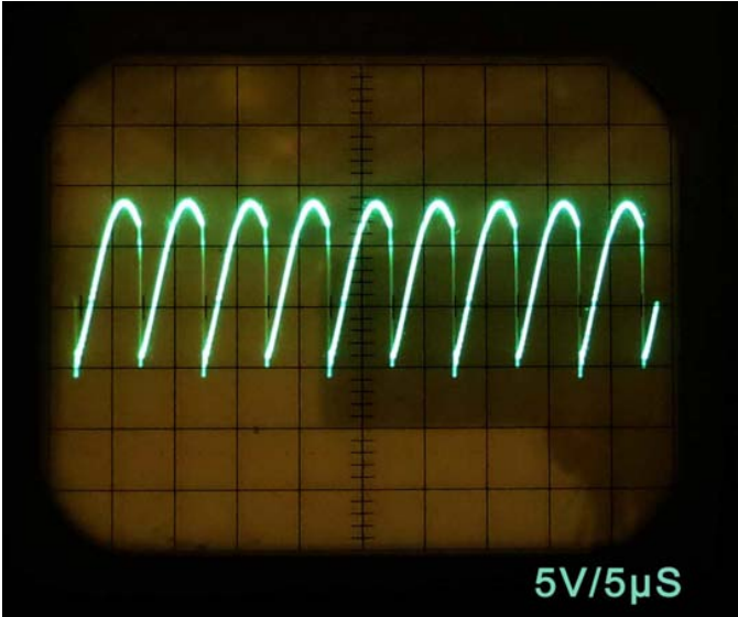
Center tap of T1/L4
