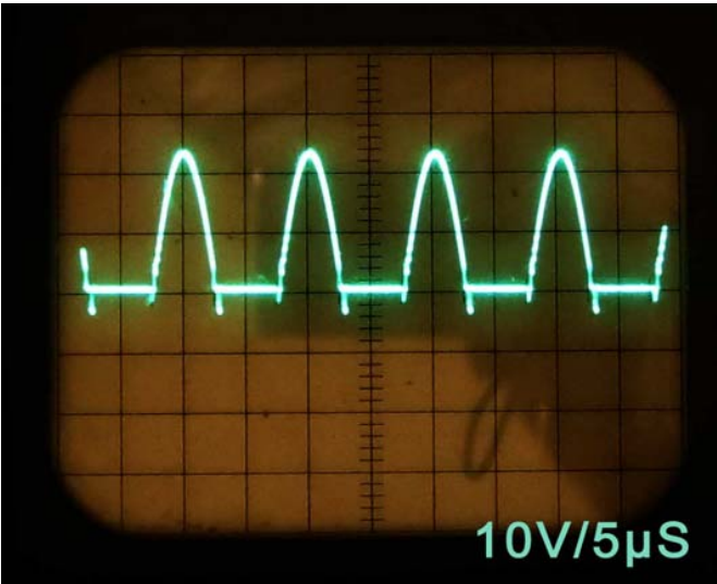
Cathode of D53, resonance tuned
