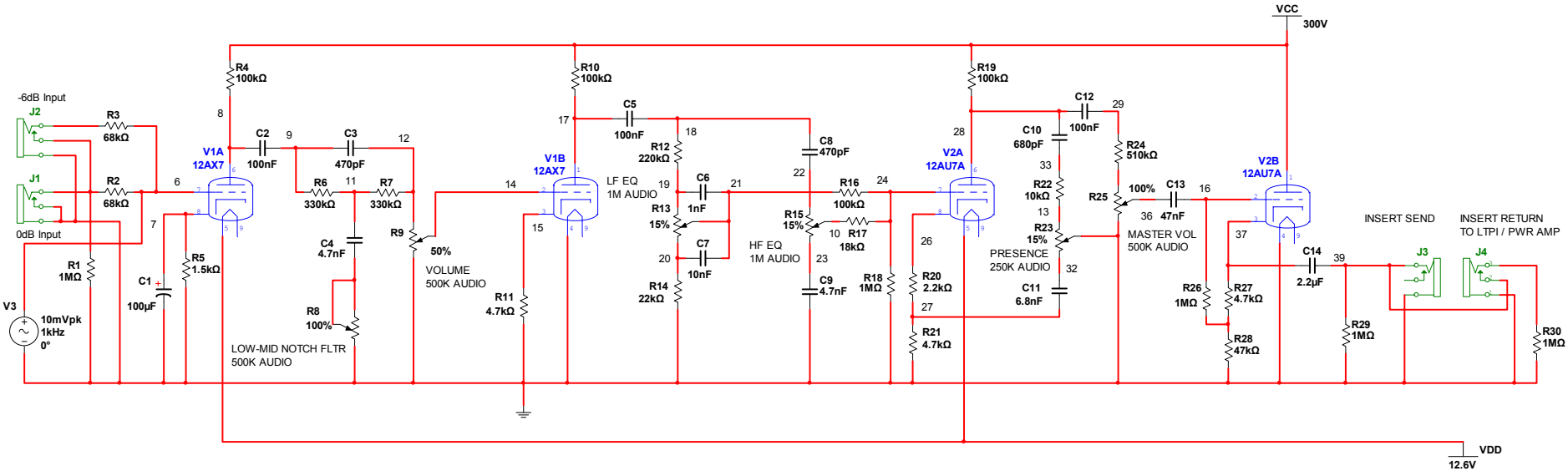
Revised Tone Control Circuit for Traynor YBA-1A
