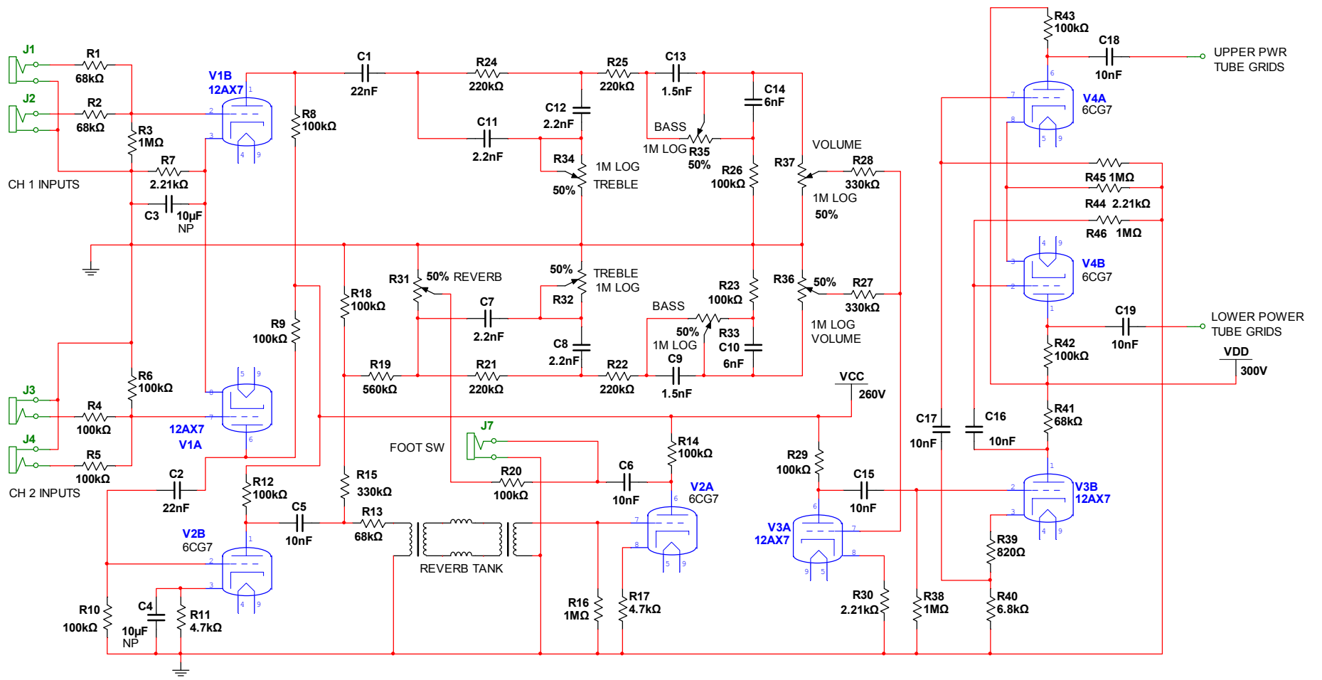
SILVERTONE 1474 PREAMP HEATER VOLTAGE FOR V1 IN SERIES WITH PWR TUBE CATODE BIAS
