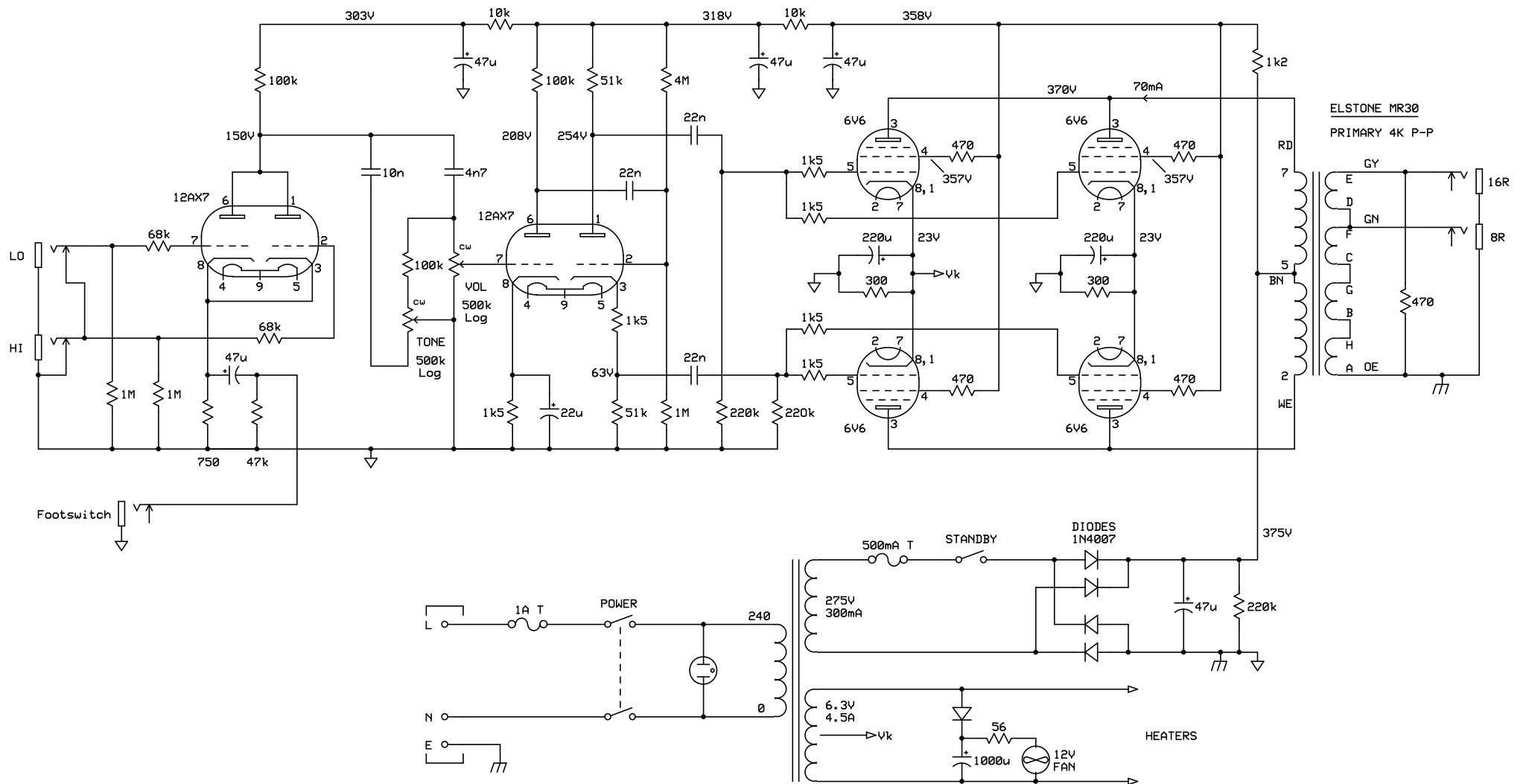
30W 6V6 GUITAR AMP
