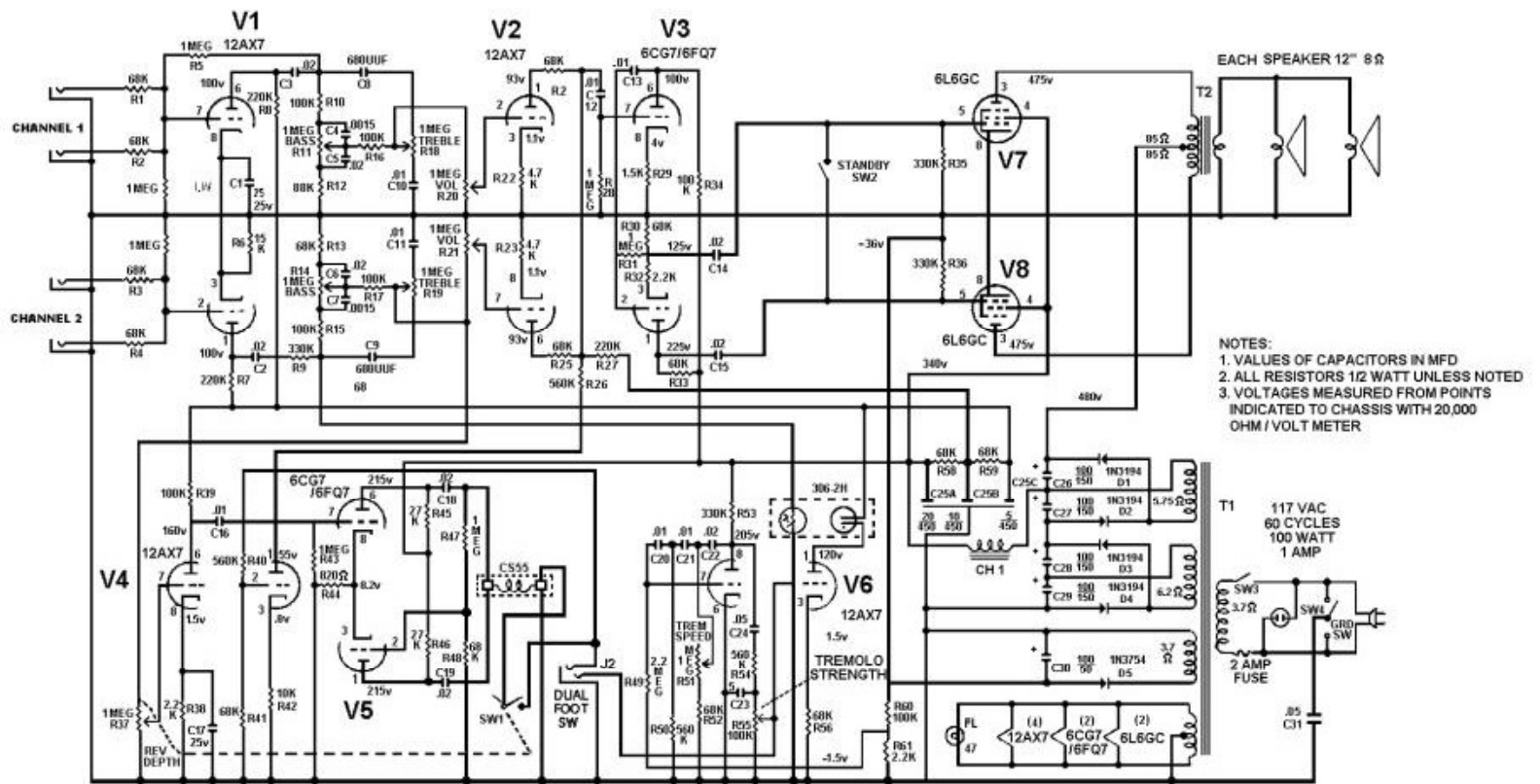
SCHMATIC DIAGRAM OF SILVERTONE CHASSIS 185.11040 MODEL 1484
