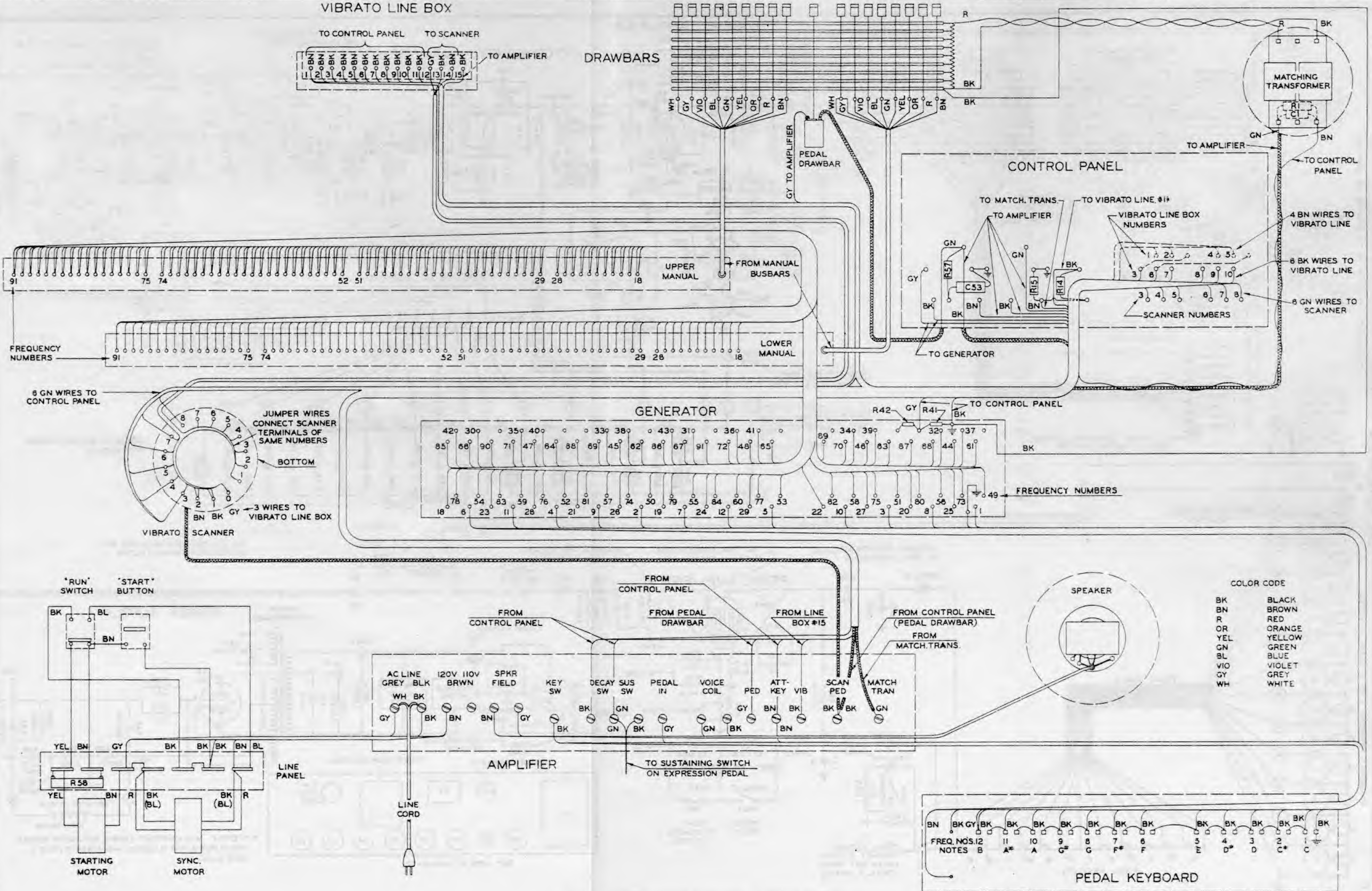
WIRING DIAGRAM MODEL M - 15083 AND ABOVE FIGURE 41A
