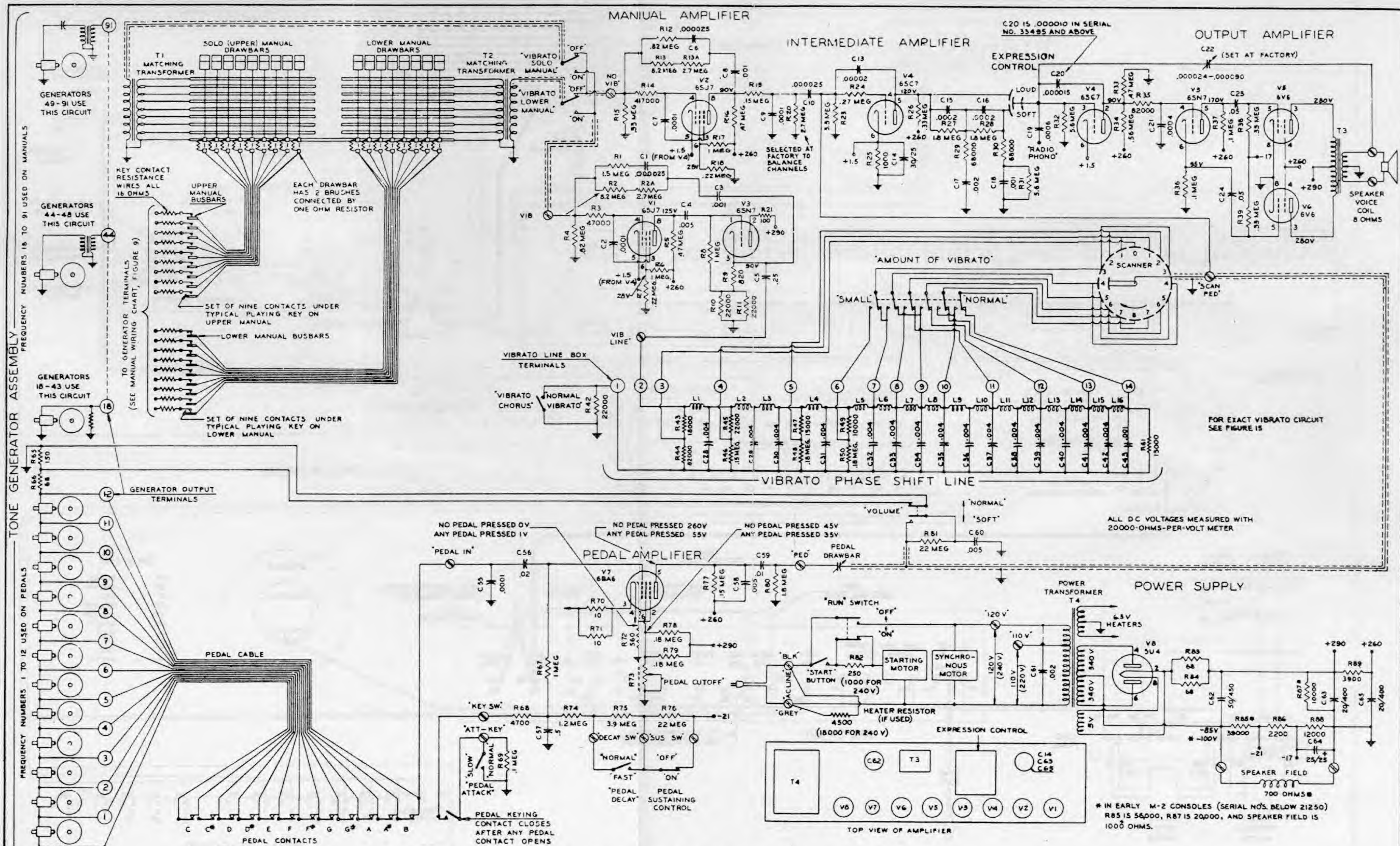
SCHEMATIC DIAGRAM MODEL M-2 - 19000 AND ABOVE FIGURE 42
