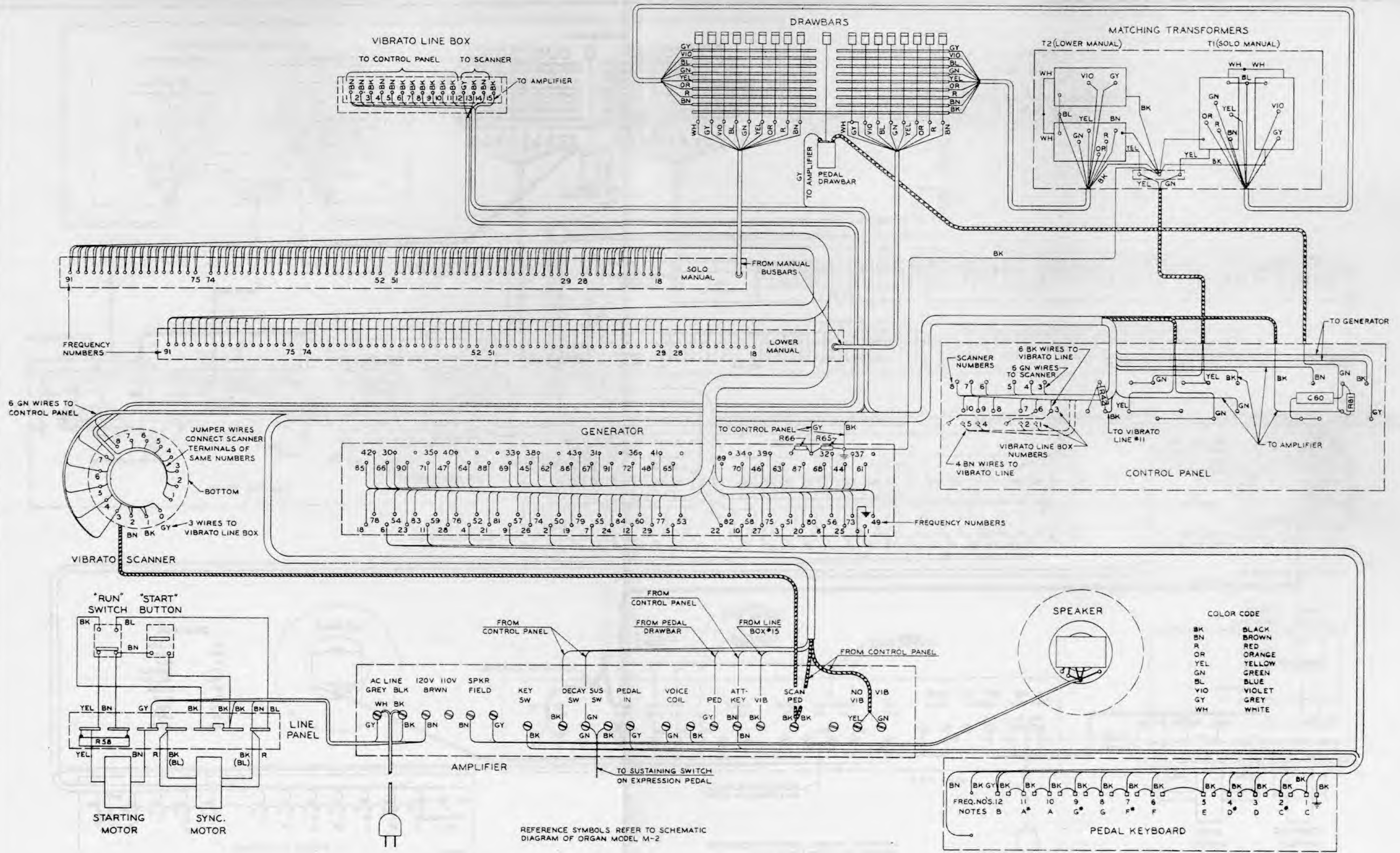
WIRING DIAGRAM MODEL M-2 - 19000 AND ABOVE FIGURE 43
