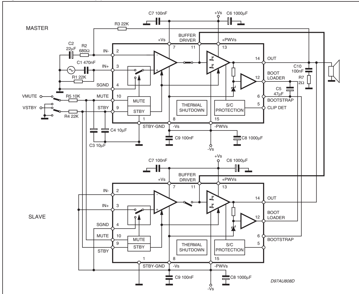
Figure 11. Modular application circuit
