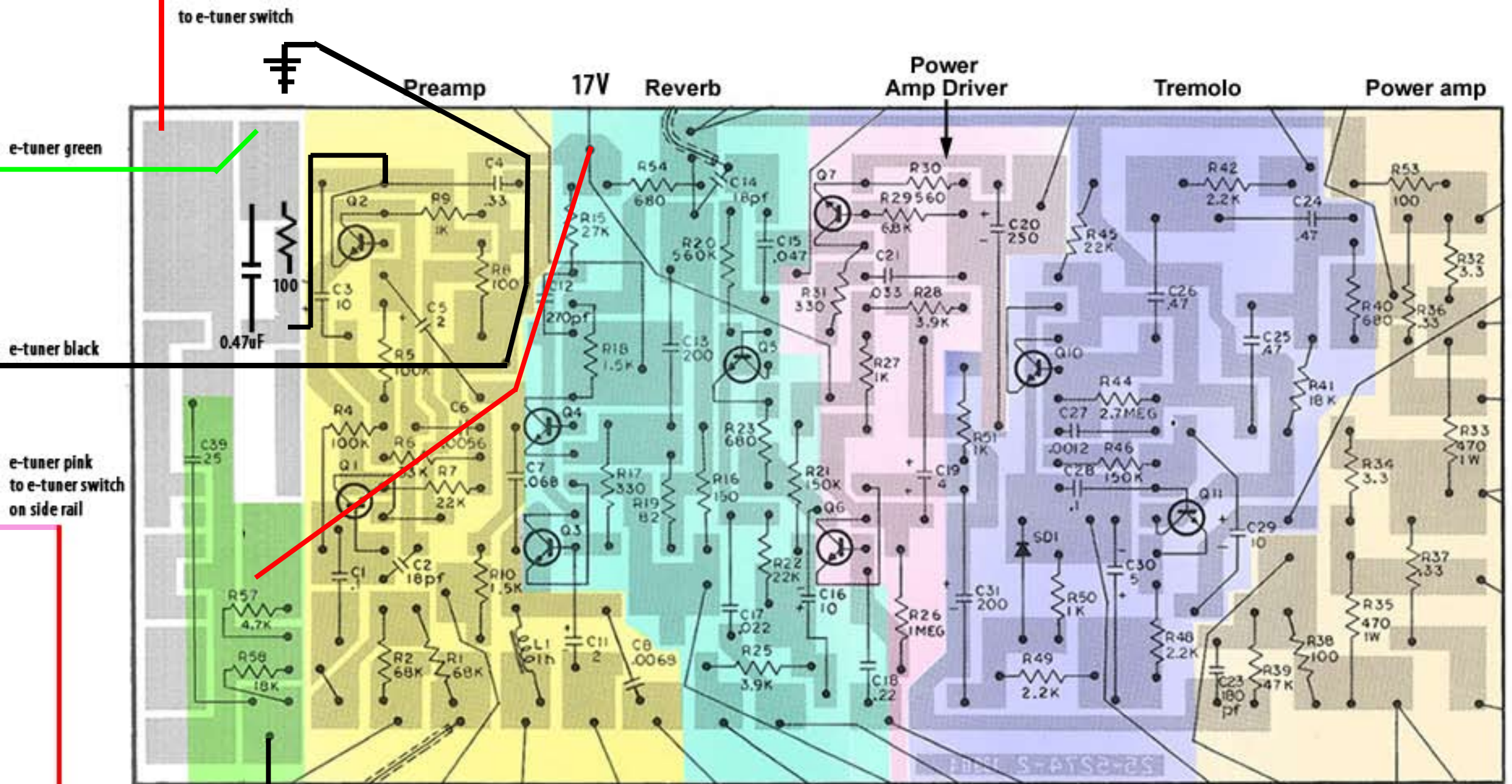
Diagram Above Shows the Thomas Organ/Vox Modular Circuit Board 25-5274-2 Populated With The Components Needed to Build a V1031 Cambridge Reverb, V1032 Cambridge Reverb or V1081 Berkeley II Amplifier. Illustration Drawn Component Side Up.
