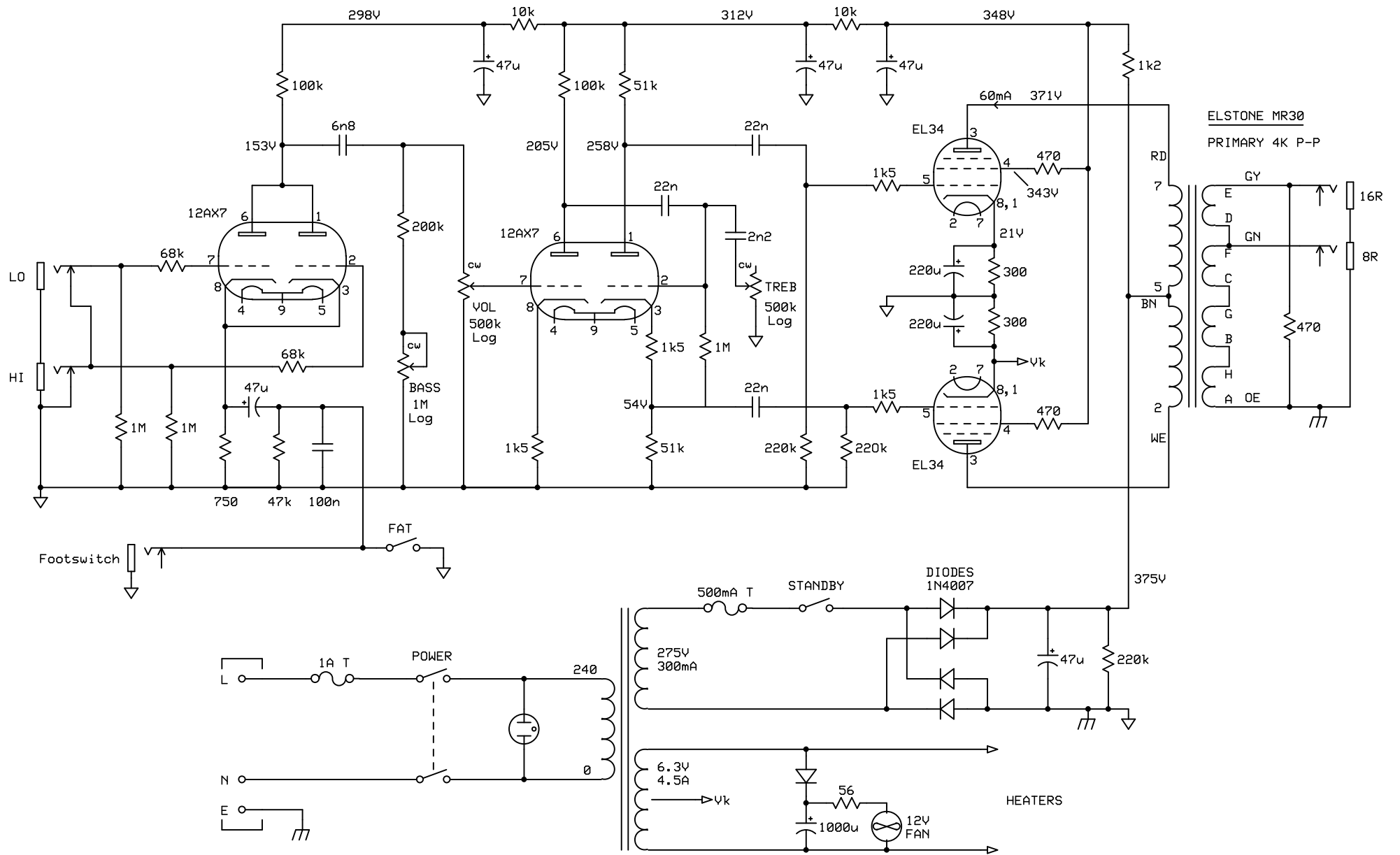
30W EL34 GUITAR AMP
