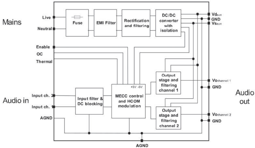
Figure 1: ICEpower50ASX2 block diagram
