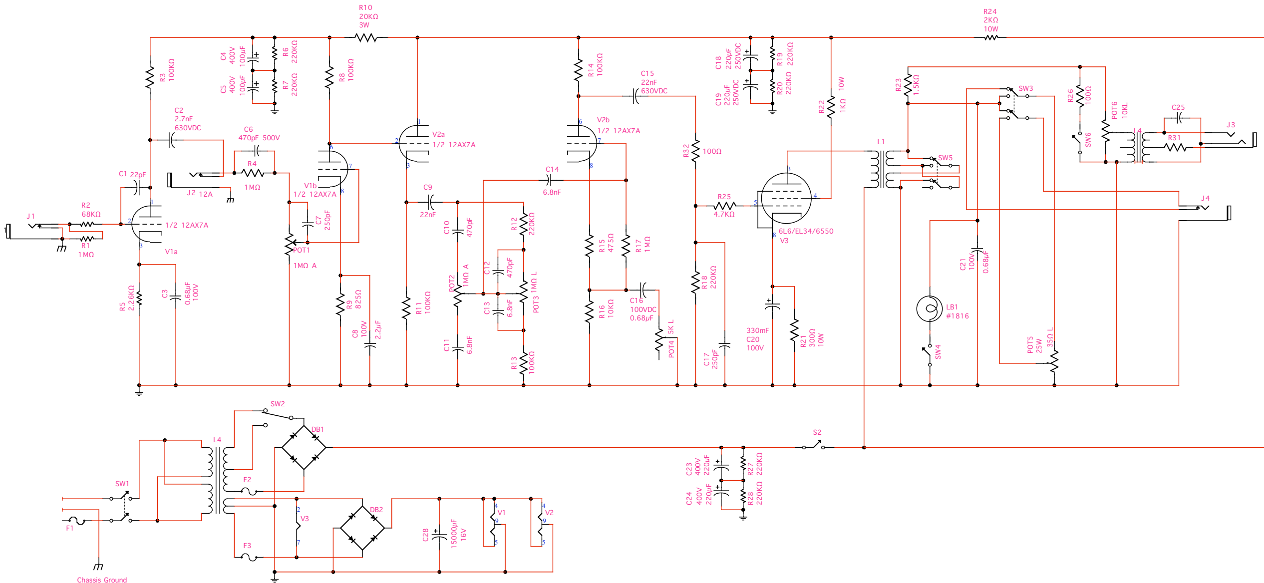
THD UniValve Schematic Version 1.41 06/21/04
