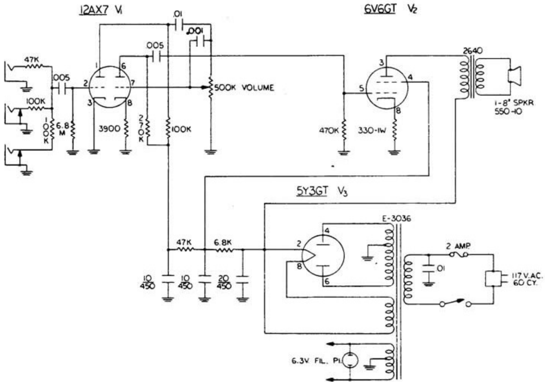
Valco Model 6150
