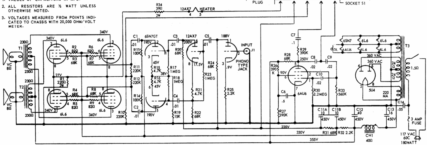
SILVERTONE MUSICAL INSTRUMENT AMPLIFIER MODEL 1396, Ch. 185.10500
