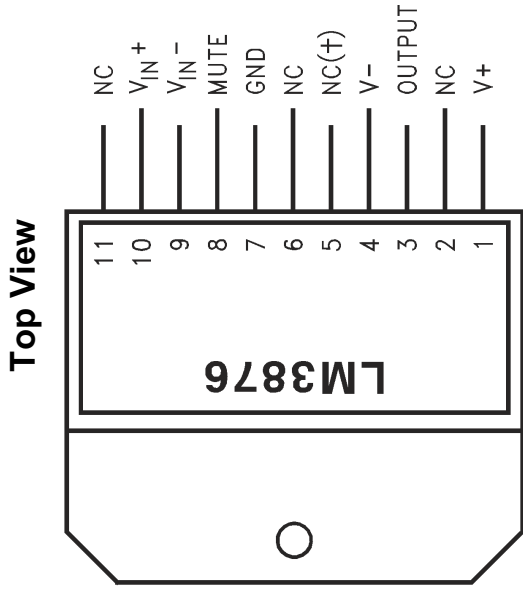
Figure 2. TO-220 and PFM Plastic Packages See Package Numbers NDJ0011B and NDA0011B (1)
