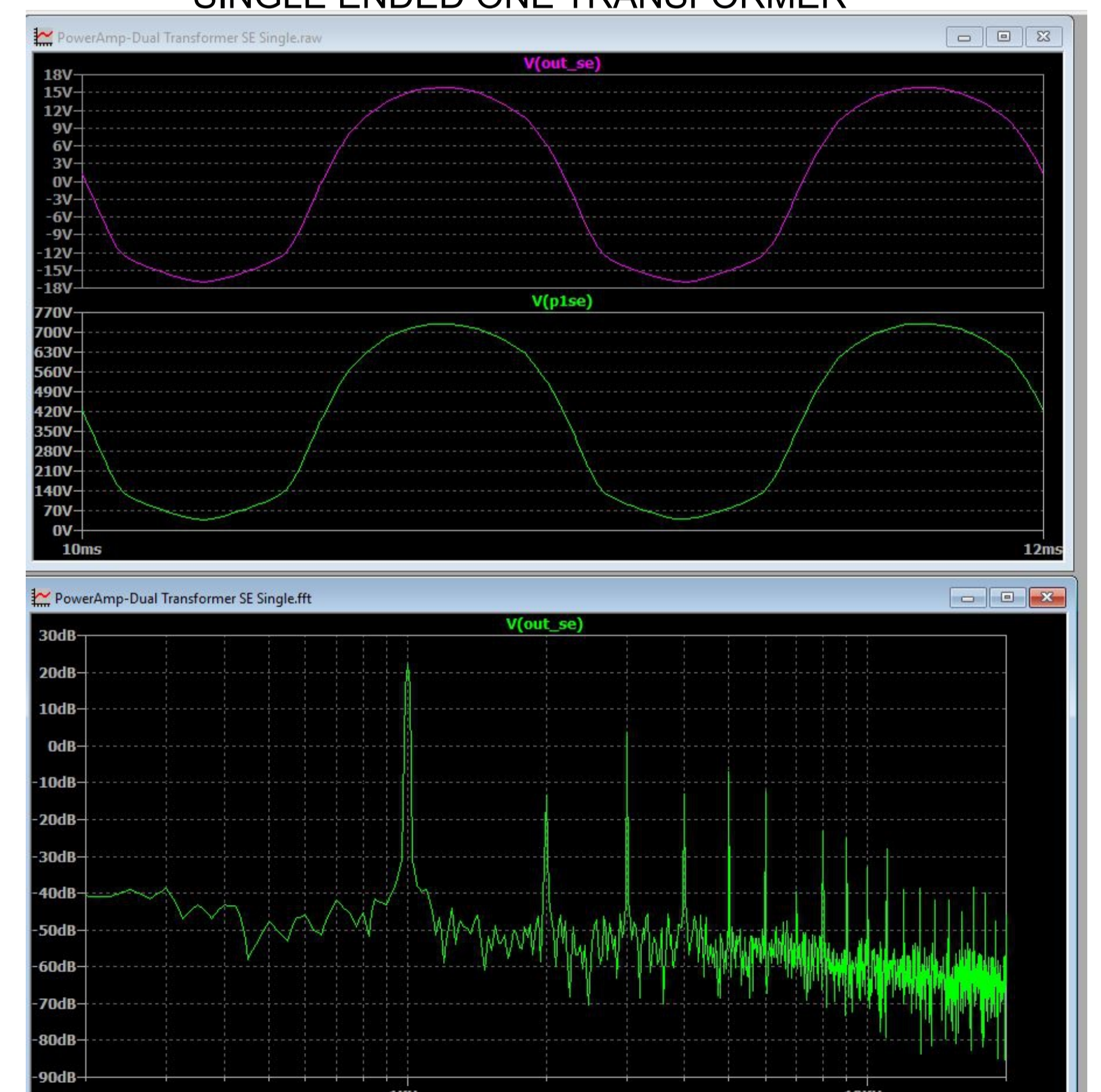
SINGLE ENDED ONE TRANSFORMER
