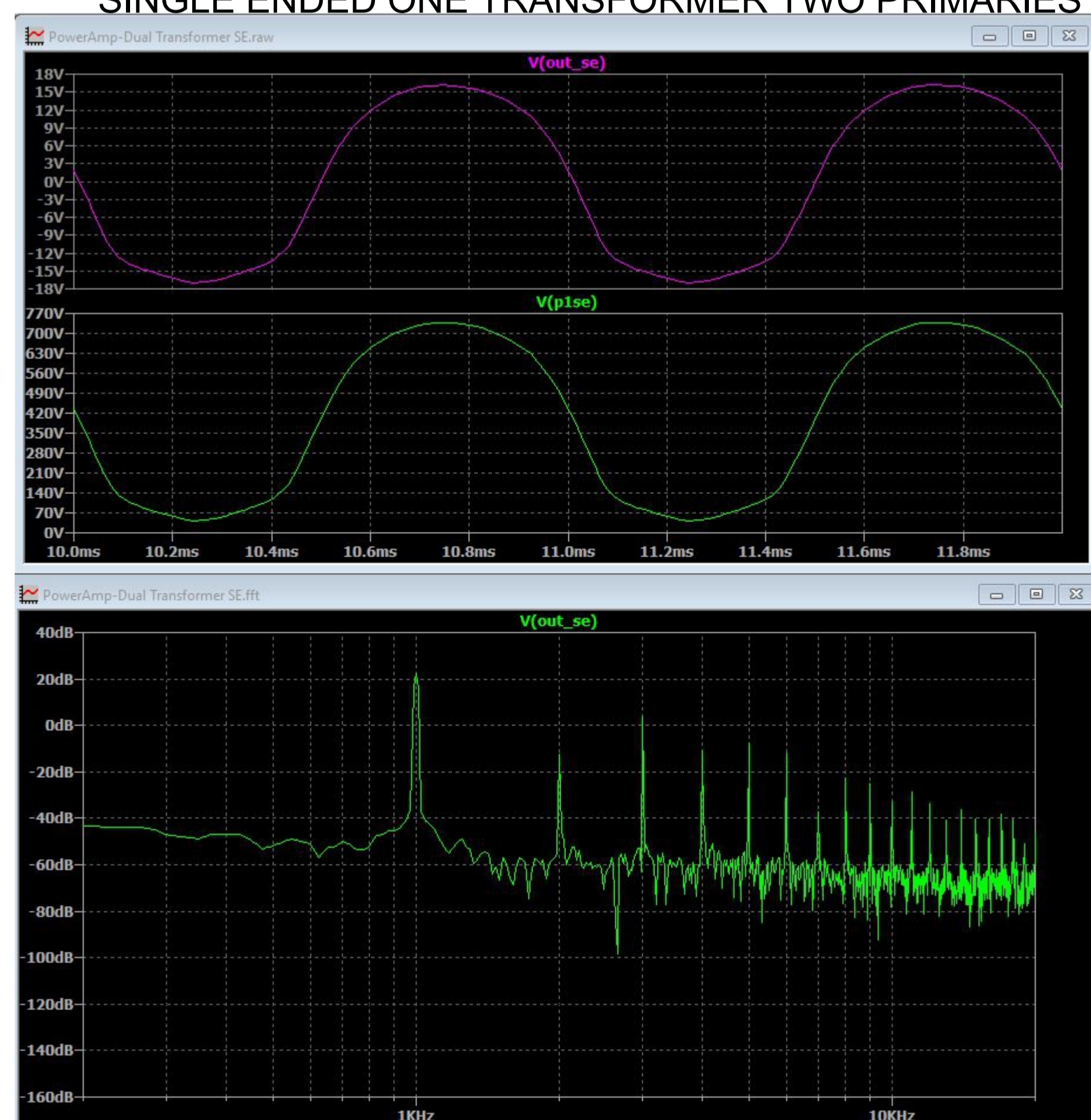
SINGLE ENDED ONE TRANSFORMER TWO PRIMARIES
