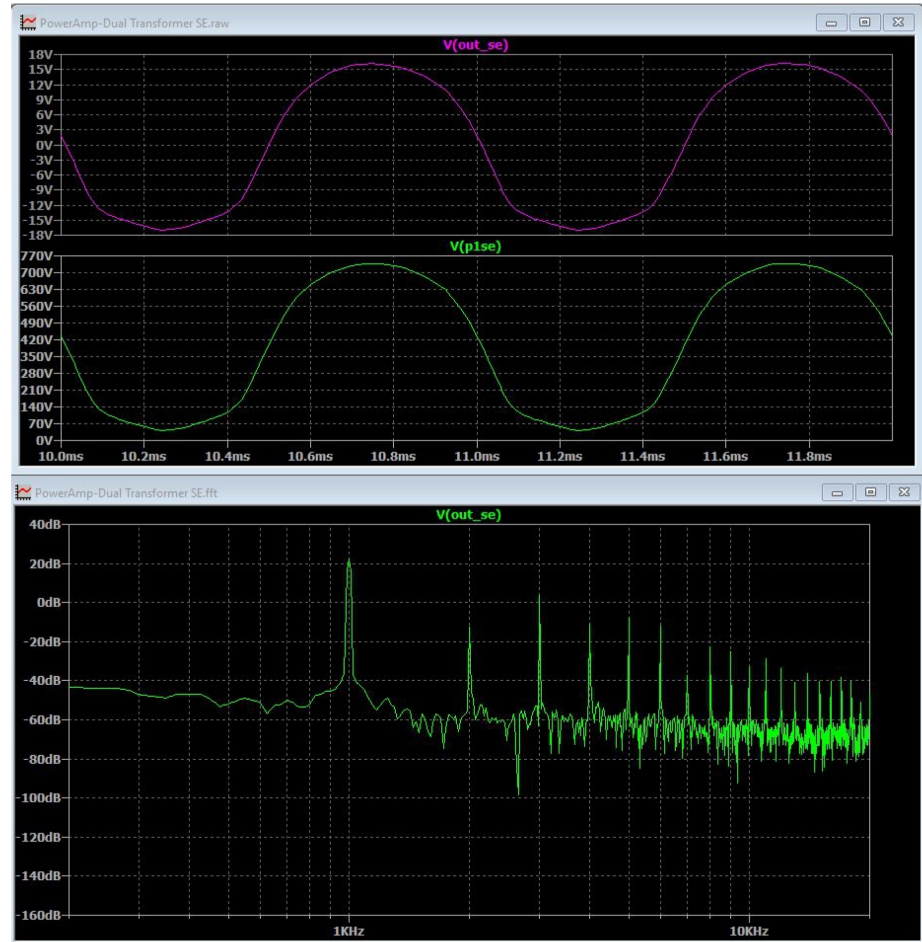
SINGLE ENDED TWO TRANSFORMERS IN PARALLEL
