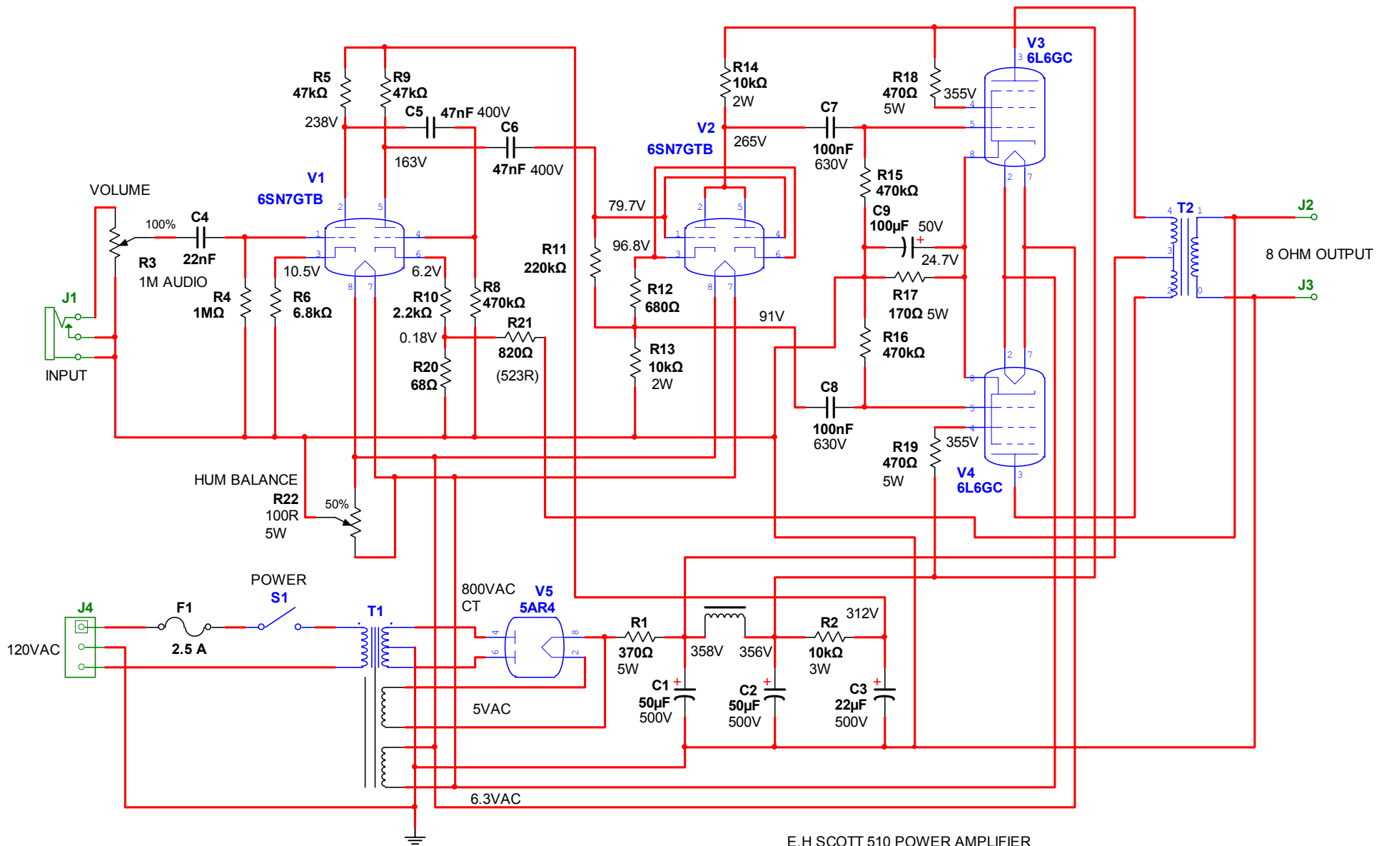
E.H SCOTT 510 POWER AMPLIFIER ONE AMP HAS HIGHER GAIN, NEEDING DIFFERENT FEEDBACK VALUE FOR R21
