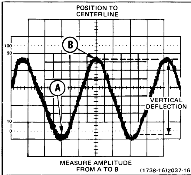
Fig. 16. Peak-to-peak voltage of a waveform.
