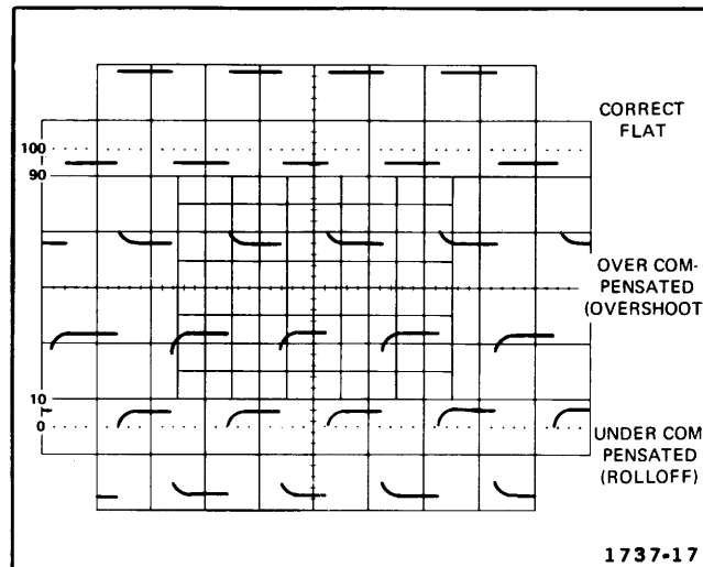
Fig. 13. Probe compensation.
