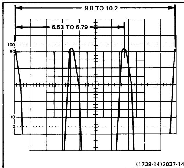
Fig. 14. Basic 466/464 timing check.
