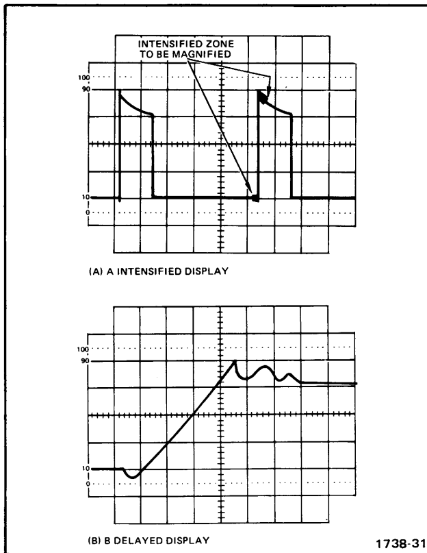
Fig. 26. Delayed sweep magnification.
