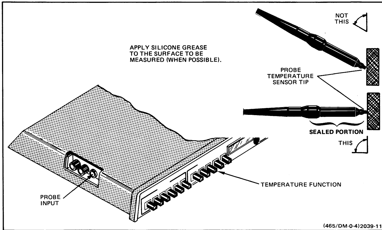
Fig. 12. Temperature.
