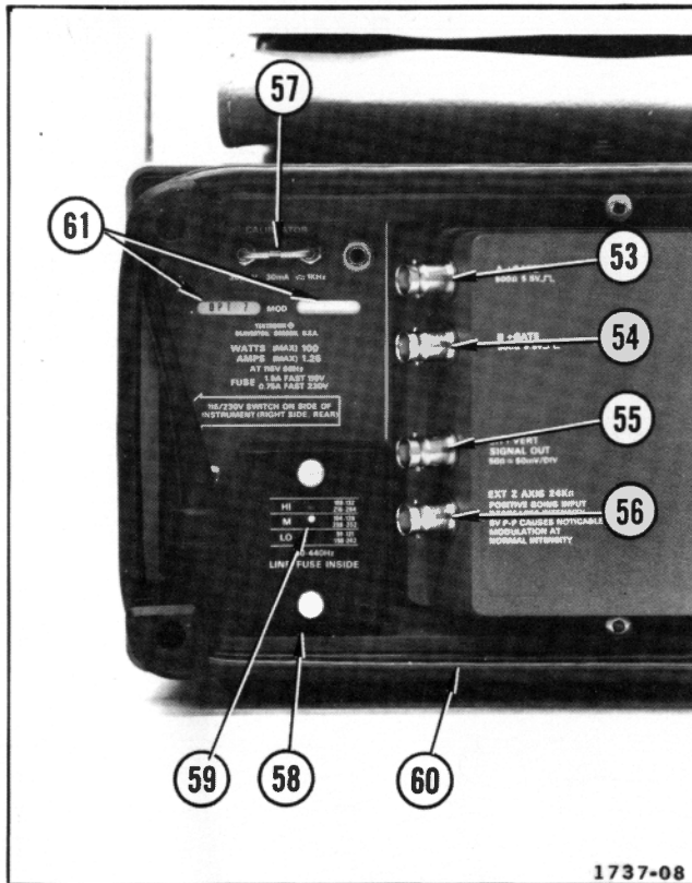
Fig. 8. Rear panel controls, connectors, and indicators.
