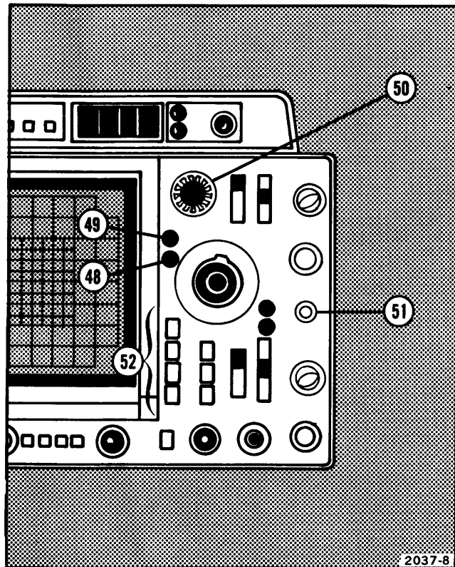
Fig. 7. Horizontal and power controls, connectors, and indicators.
