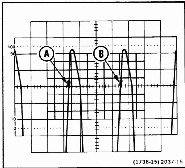
Fig. 15. DM44 timing check.
