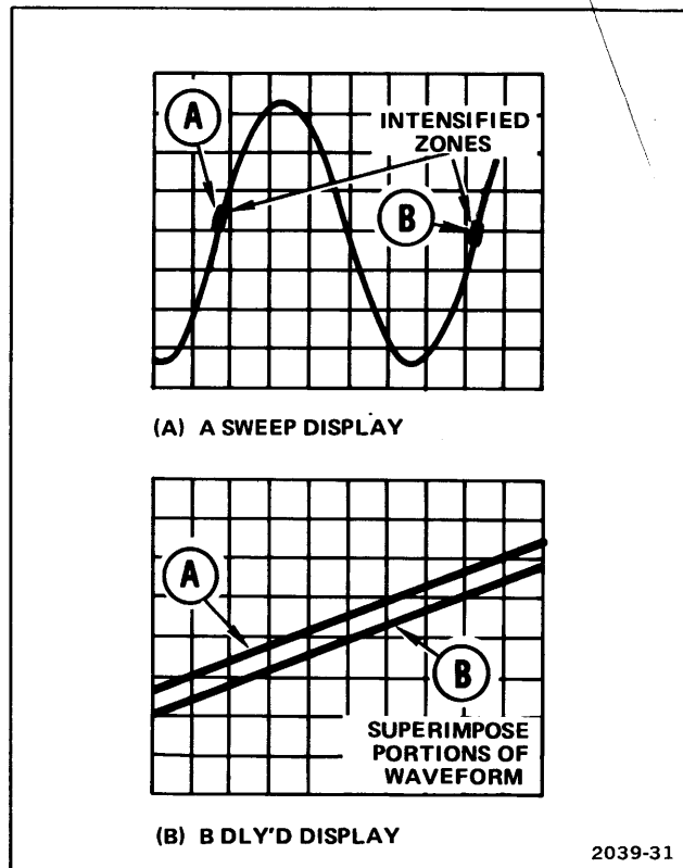
Fig. 32. Time duration and frequency measurements.
