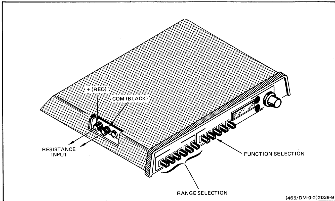
Fig. 10. Resistance.
