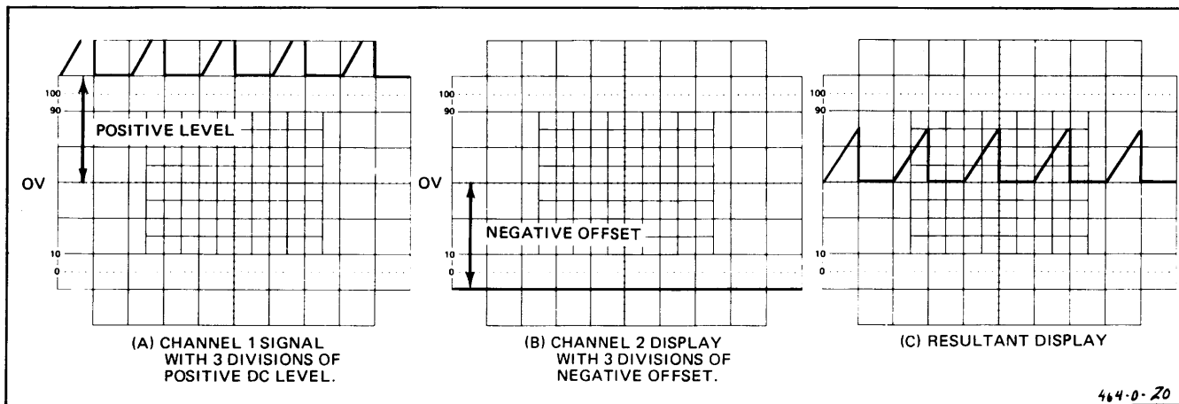
Fig. 18. Algebraic addition.
