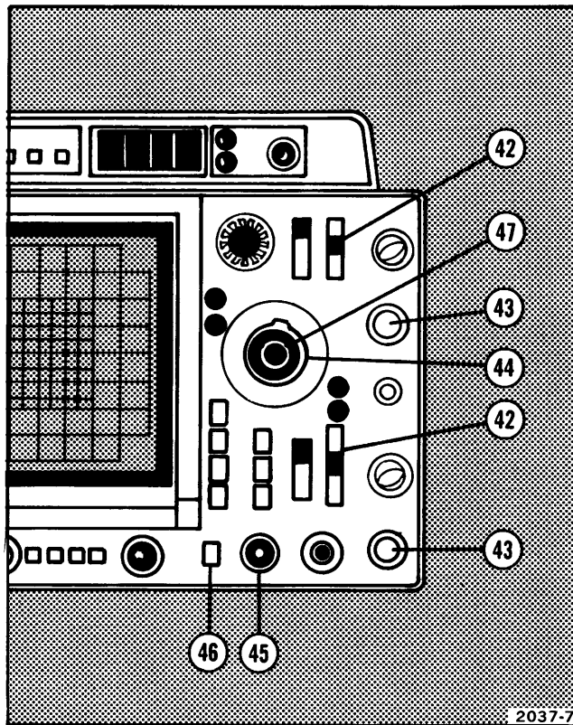
Fig. 6. Trigger, horizontal, and power controls, connectors and indicators.
