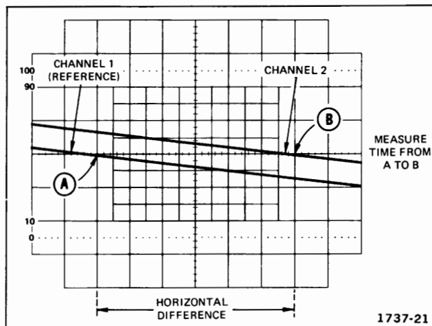
Fig. 24. High-resolution phase difference.
