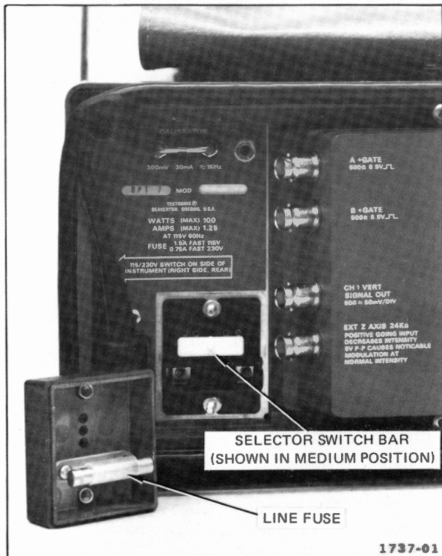
Fig. 1. Regulating range selector & line fuse.
