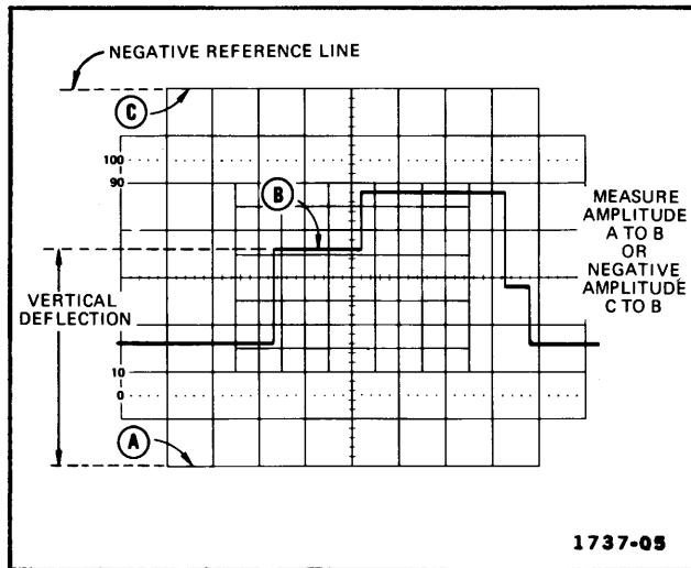
Fig. 17. Instantaneous voltage measurement.
