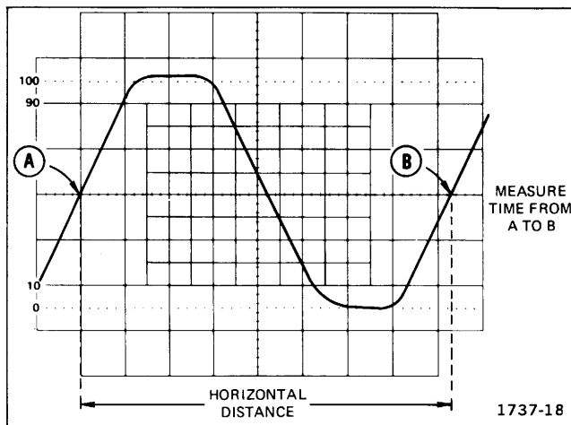
Fig. 20. Time duration.
