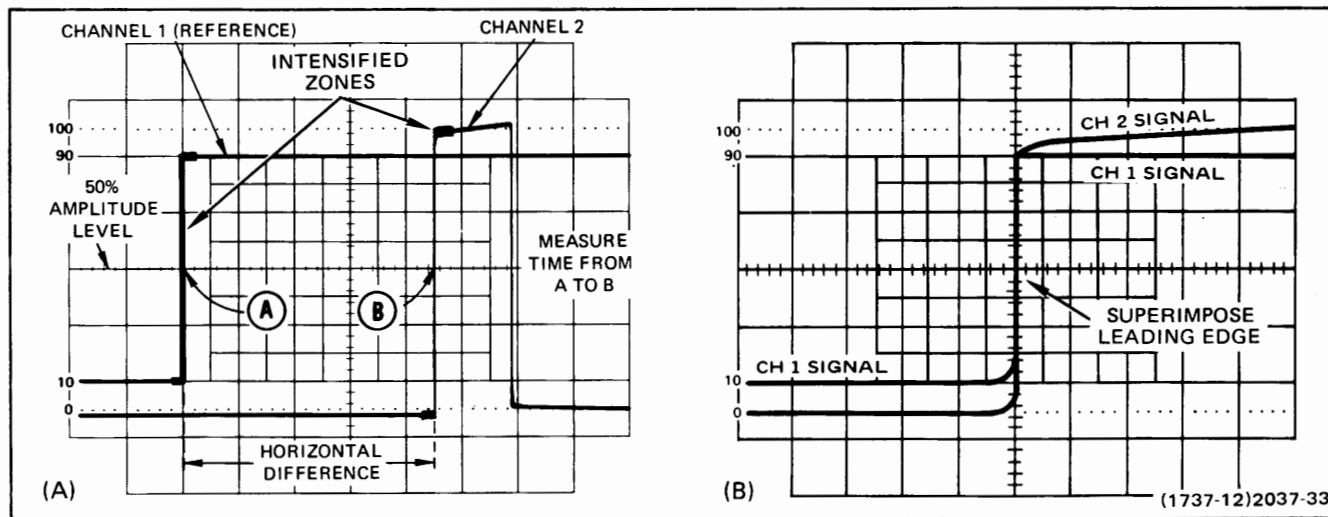
Fig. 33. Time difference between two pulses from different sources.
