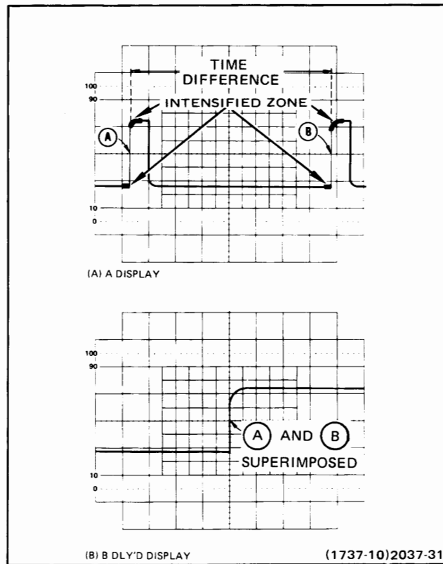
Fig. 31. Time difference between repetitive pulses.
