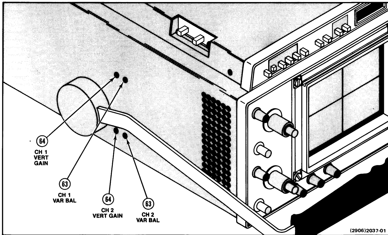
Figure 8A. Left side panel controls.
