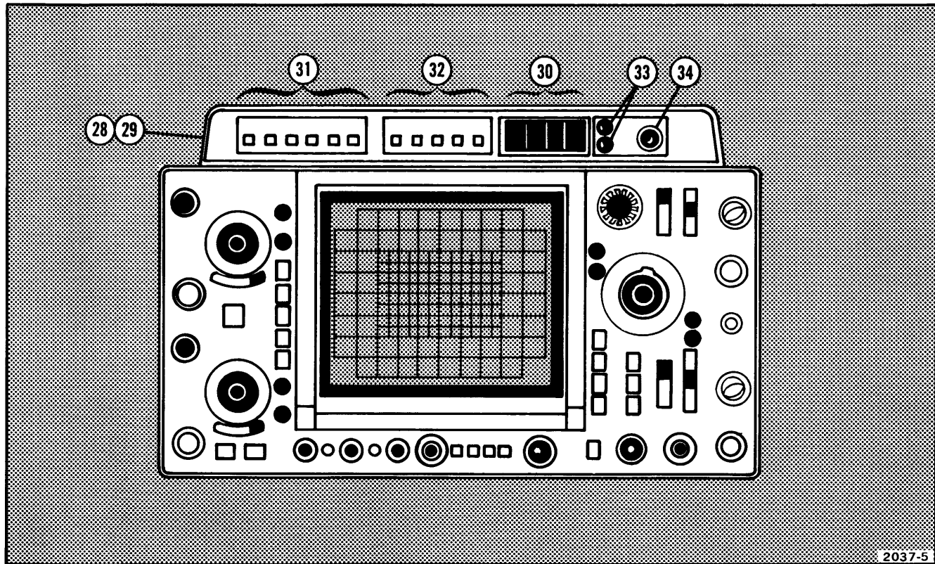
Fig. 4. DM44 controls, connectors, and indicators.
