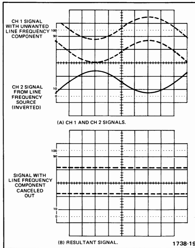
Fig. 19. Common-mode rejection.
