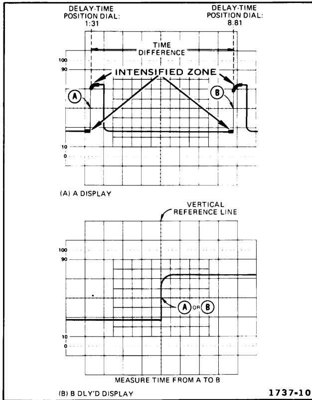
Fig. 27. Time difference between repetitive pulses.
