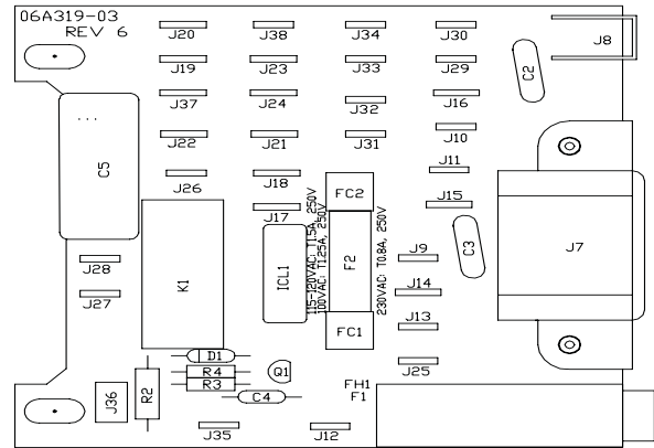
< AC TERMINATION >
