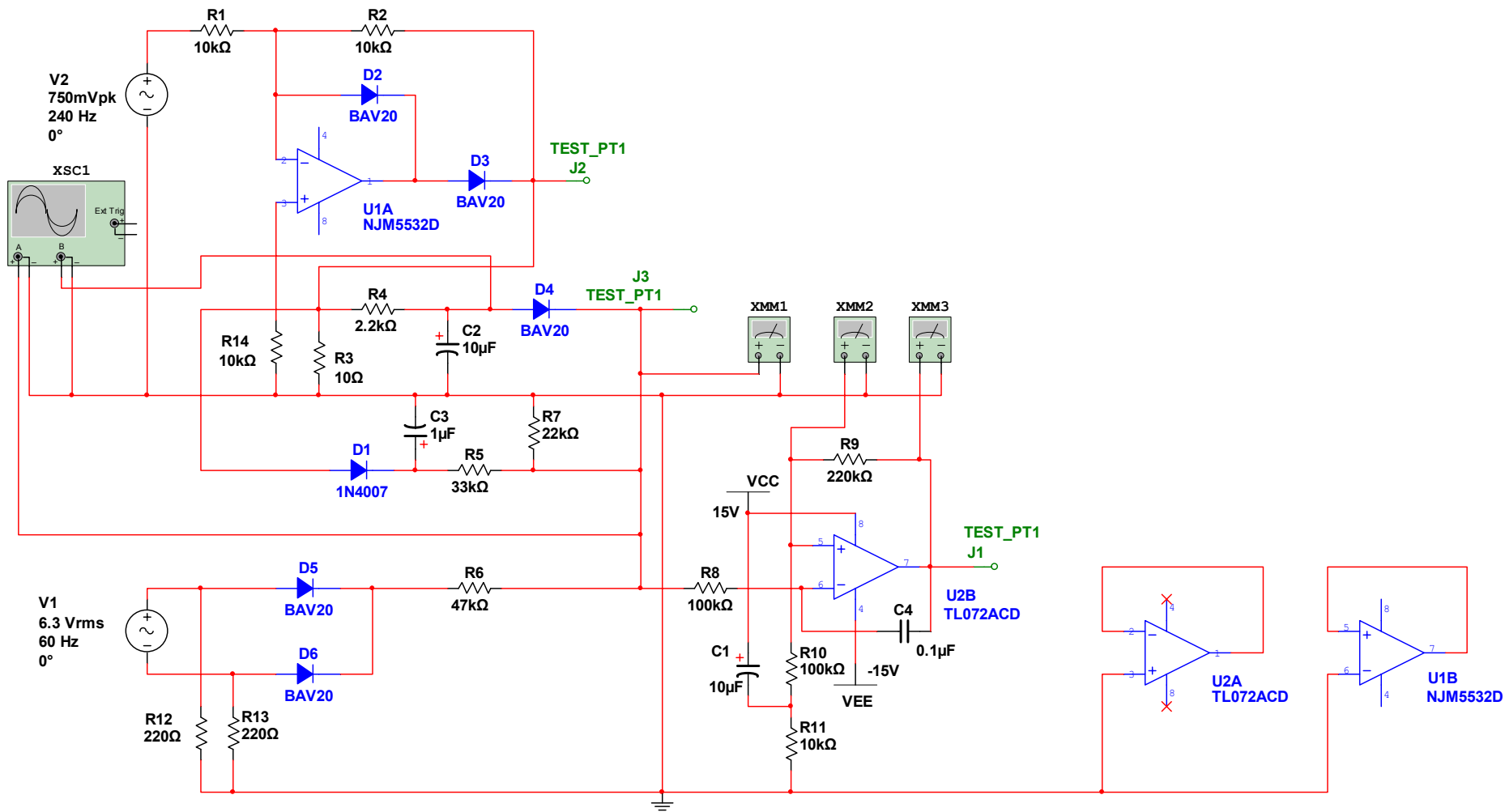
SVT-CL FAULT DETECTION CIRCUIT, SIMPLIFIED
