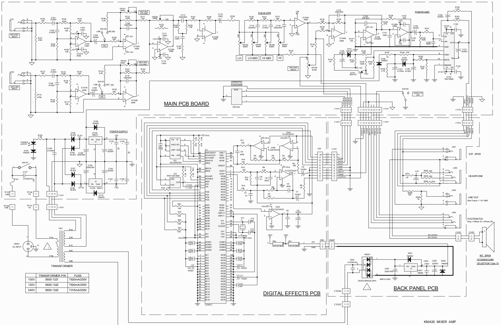
KMA35 MIXER AMP
