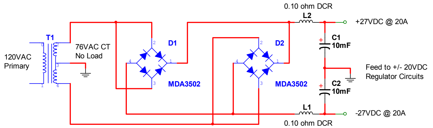
ATI PARAGON PPS1 UNREGULATED POWER SUPPLY BRIDGE RECTIFIER CIRCUIT
