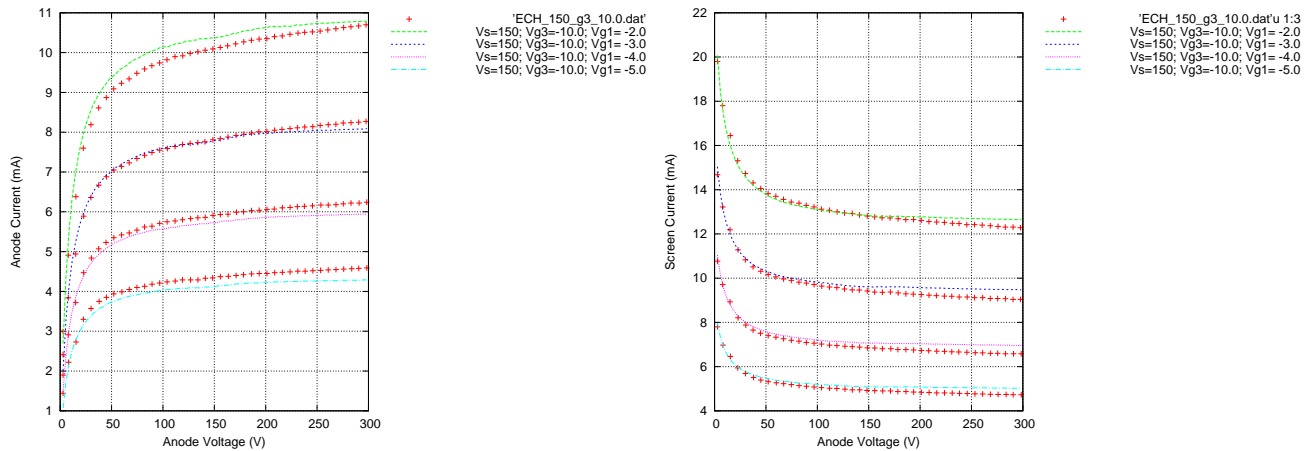
Figure 15: Left: Anode current I_a for an ECH81, with V_{g2} = V_{g4} = 150V , and for V_{g1} = -2, -3, -4, -5V . Right: the same, but for I_{g2} + I_{g4} .
