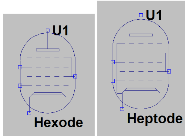
Figure 11: Left: Hexode symbol (created in LTSpice) representing the model development in Sec. 6. Right: the corresponding heptode symbol.
