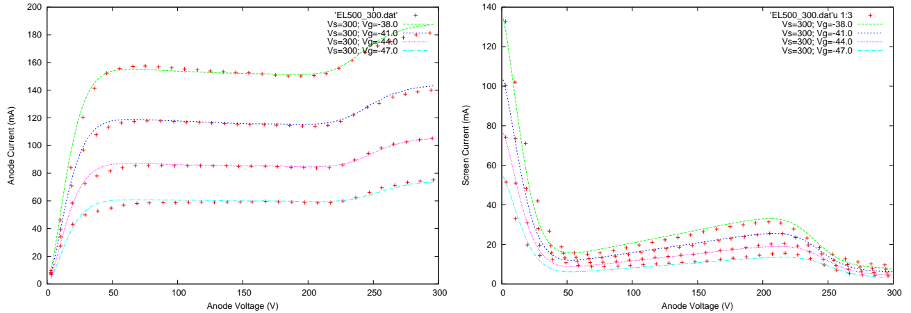
Figure 10: Model fits of anode and screen current of a EL500 according to the model of Sec. 5.4.
