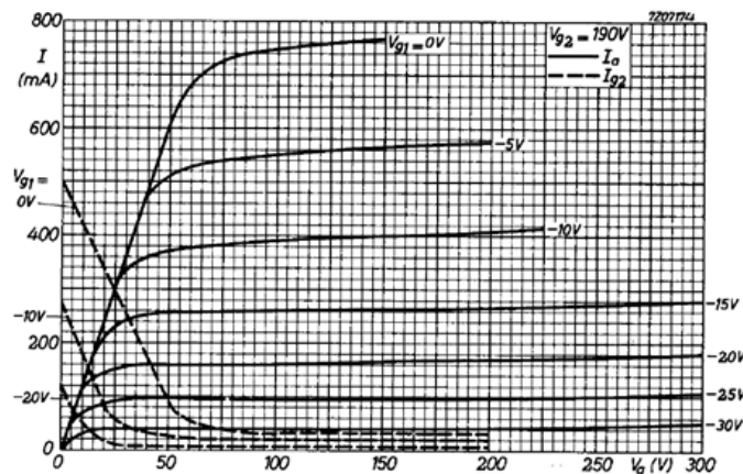
Figure 7: Anode current of a EL500/PL504 according to the Philips datasheet.
