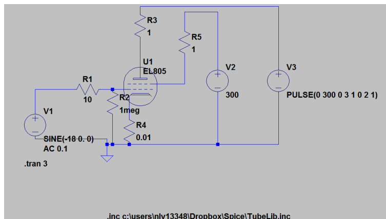
Figure 20: Spice test circuit for the models generated by ExtractModel .
