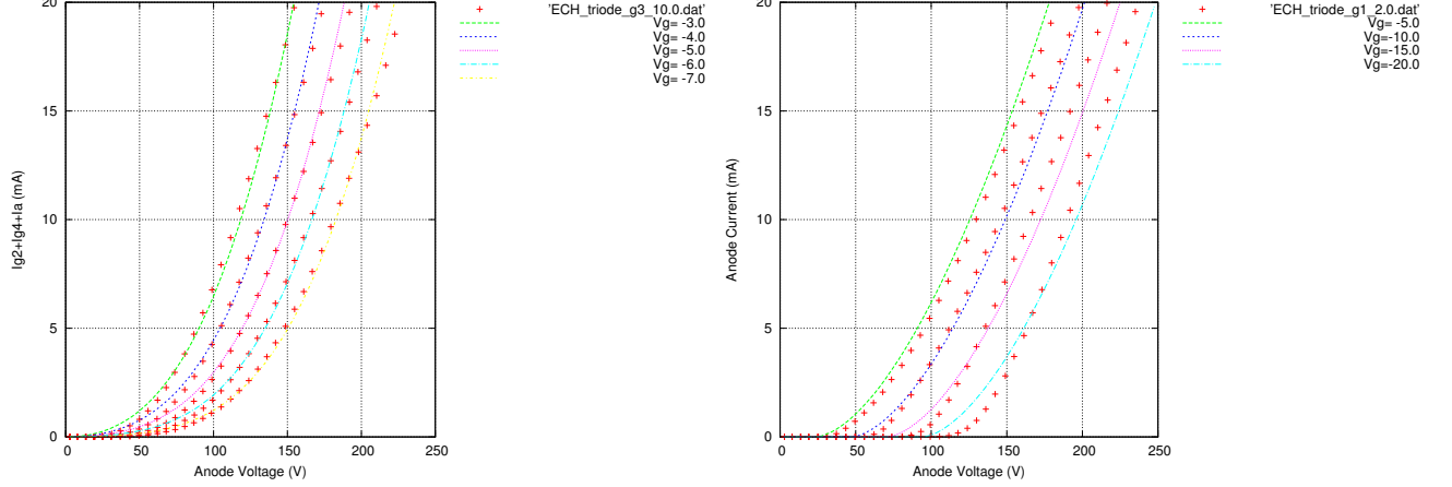
Figure 14: Left: Standard triode fit with g1 as control grid of total space current I_c at V_{g3} = -10V . Right: Standard triode fit with g3 as control grid of the anode current at V_{g1} = -2V .
