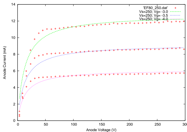
Figure 5: Model fits of anode current of a EF80 according to the model of Sec. 4.4.
