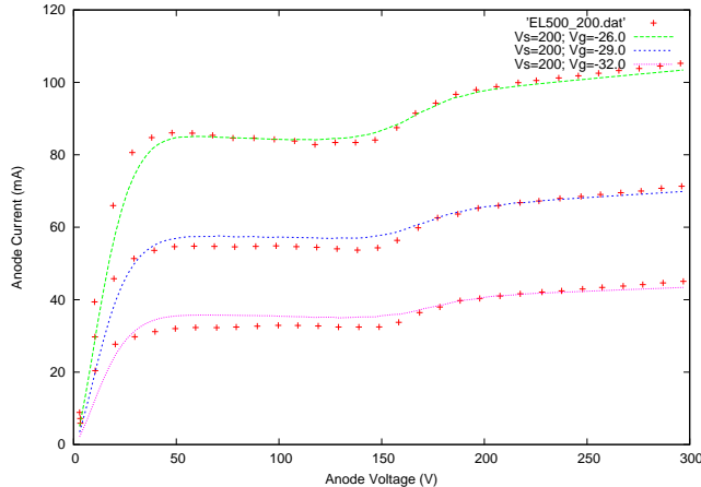
Figure 8: Anode current of a EL500/PL504 as measured with the uTracer. The drawn lines are fits based on the model presented in Sec. 5.4.
