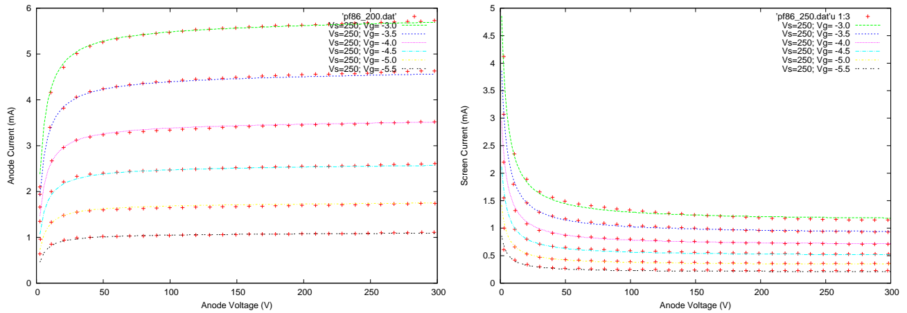
Figure 4: Model fits of anode and screen current of a PF86 according to the model of Sec. 4.4.
