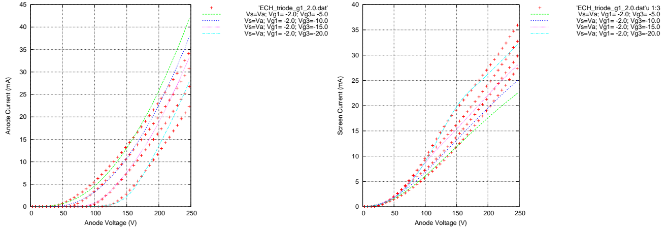
Figure 16: Left: Anode current I_a for an ECH81, with V_a = V_{g2} = V_{g4} , and for V_{g3} = -5, -10, -15, -20V . Right: the same, but for the total screen current I_{g2} + I_{g4} .
