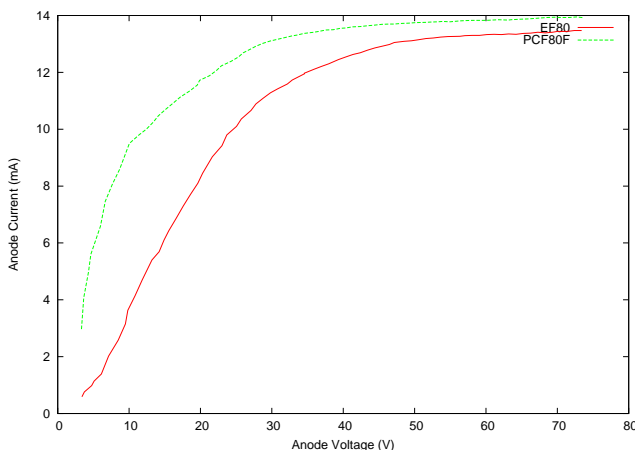
Figure 23: Low anode voltage behaviour of the anode current for an EF80 and PCF80(F).
