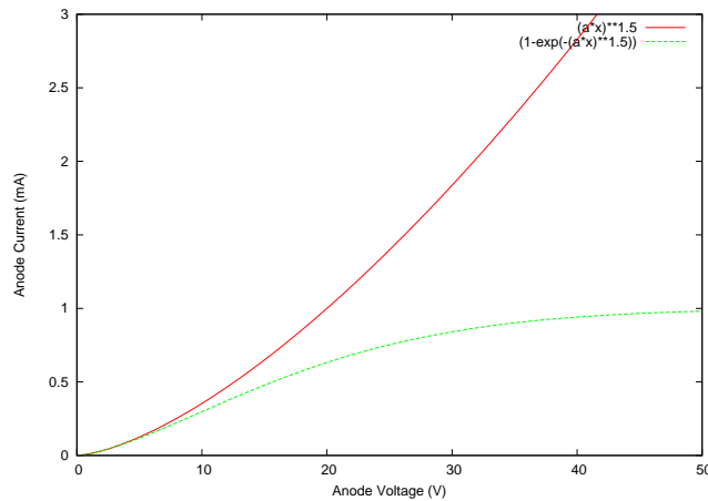
Figure 24: Modelling the low anode voltage behaviour of the virtual diode. In red, the power (3/2) behaviour; in green the behaviour including saturation ('kink').
