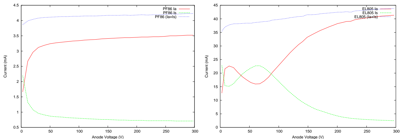
Figure 22: Demonstration of constant space charge for the EL805.
