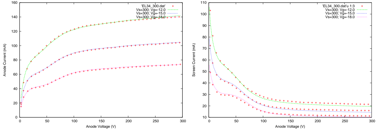
Figure 9: Model fits of anode and screen current of a EL34 according to the model of Sec. 5.3.
