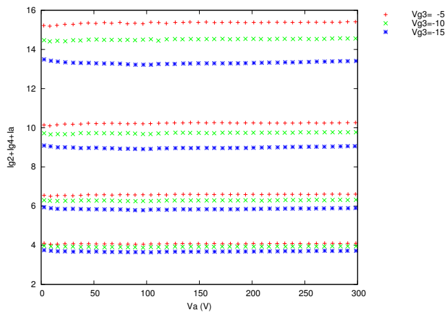
Figure 12: Space current for an ECH81 at V_{g2} = V_{g4} = 100V , for V_{g1} = 1, 2, 3, 4 .
