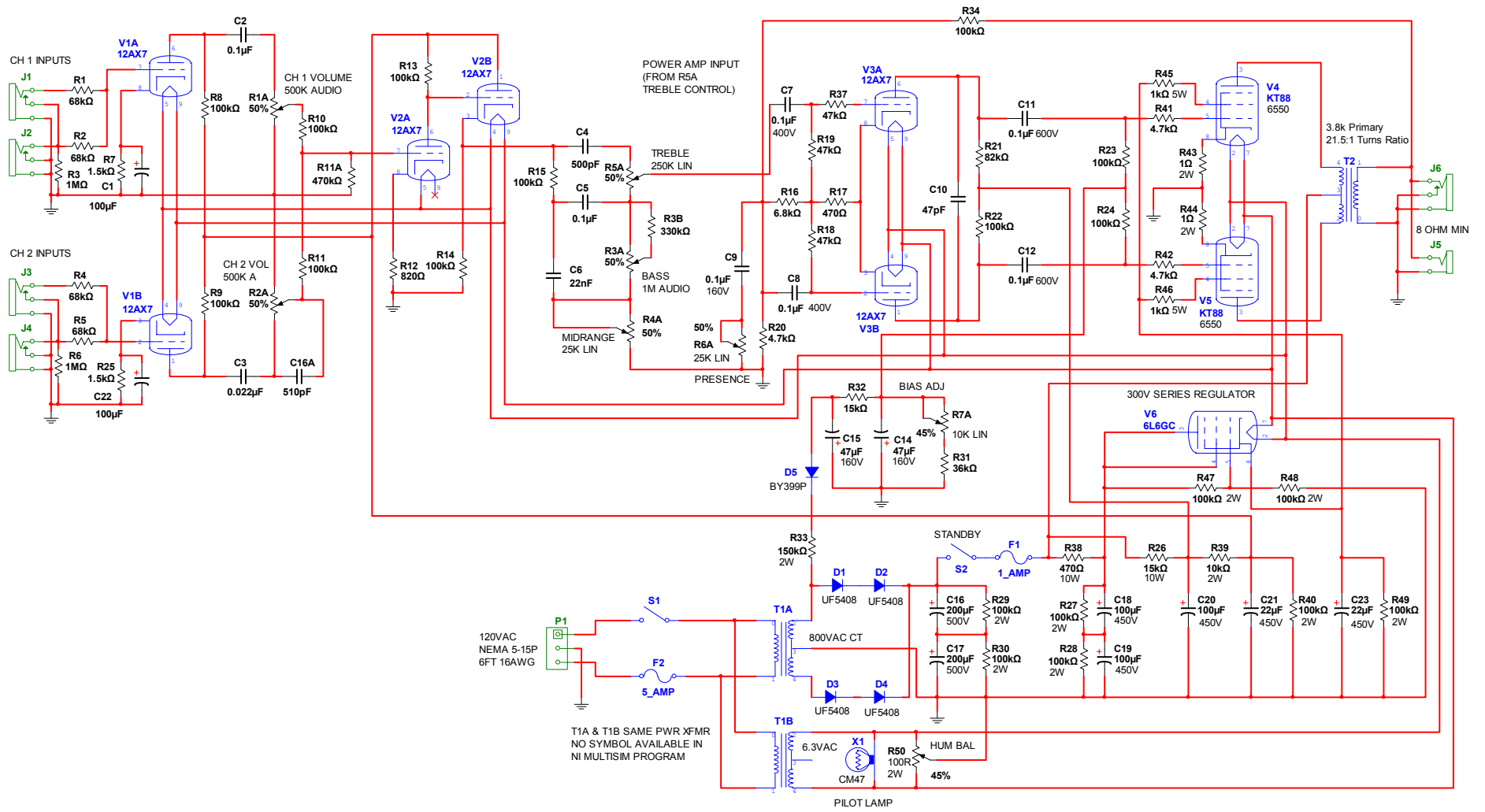
TRAYNOR YBA-1A MK II BASSMASTER CURRENT STATE OF MOD'S 8/18/14
