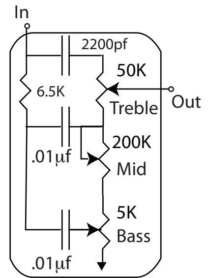
Tone Stack
