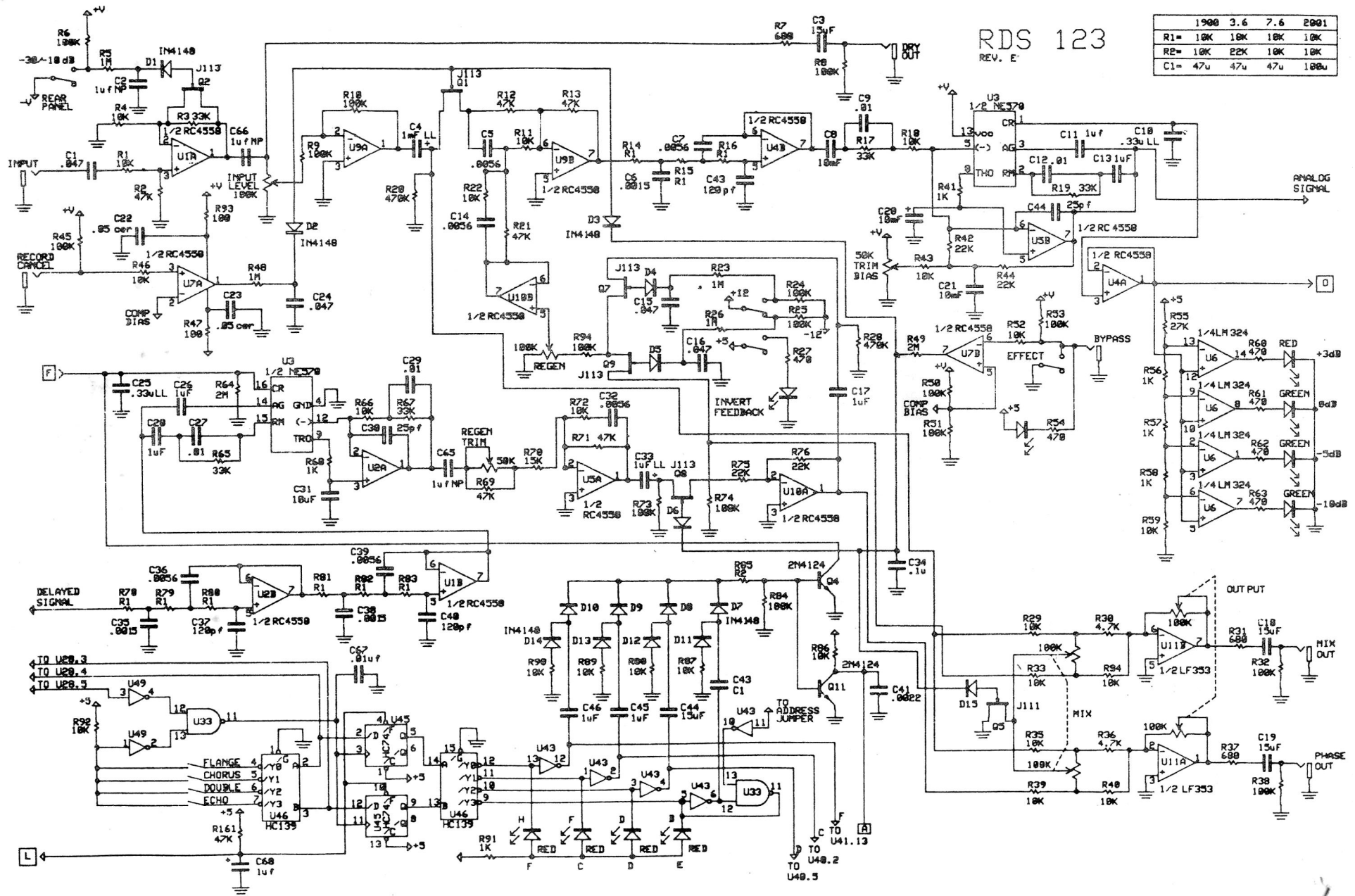
Digitech RDS 123 REV E. Schematic for RDS 1900, RDS 3.6, RDS 2001, RDS 7.6 digital delay effect processors page 1 of 2
