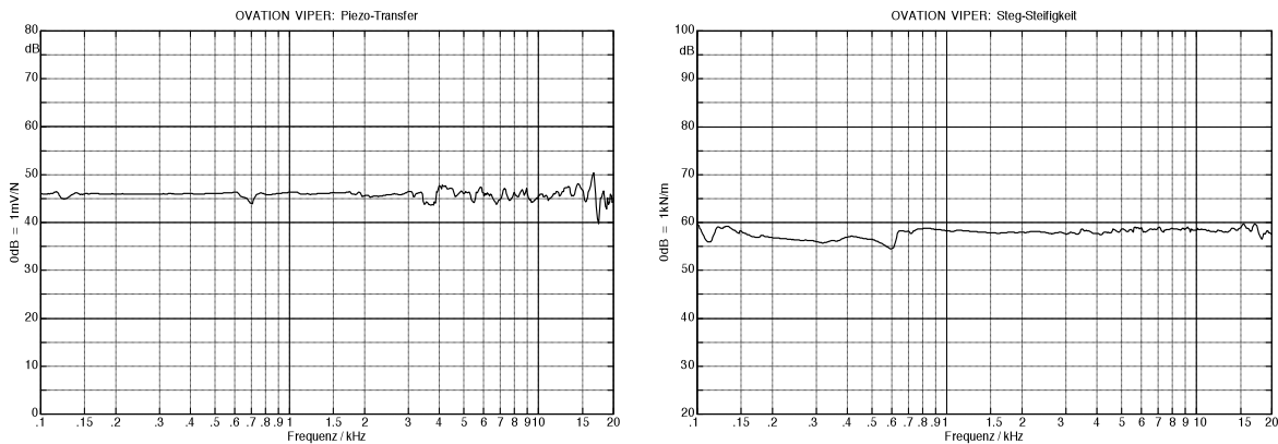
Fig. 6.7: Measurements with compensation of the measurement-head artifacts. Transmission factor (left), bridge stiffness (“Steg-Steifigkeit”, right). “Frequenz” = frequency.
