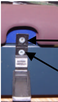
Fig 3.0 Removal Of Old Style Fixing If Required
