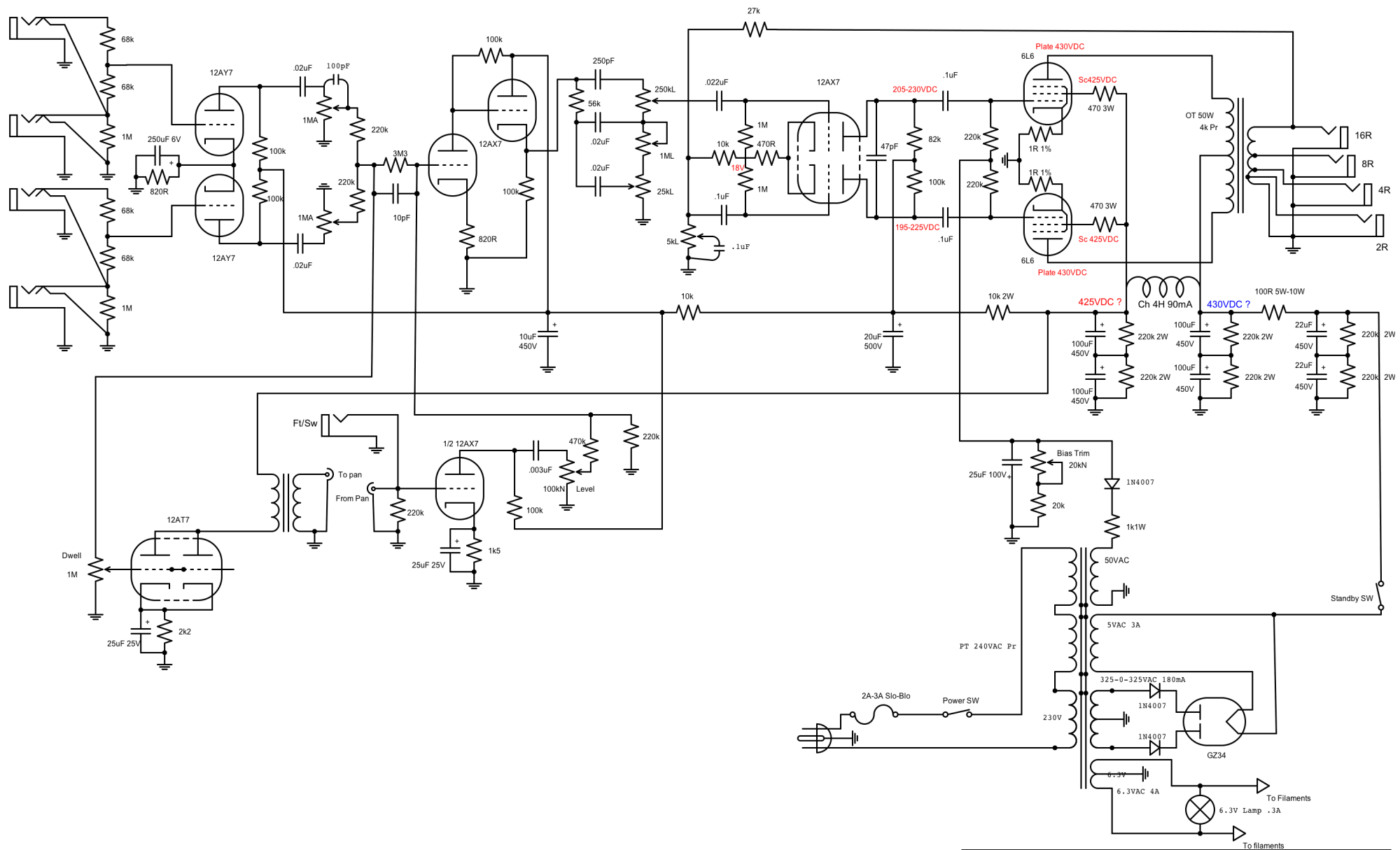
Tweed Bassman w/ Verb PR reverb circuit Tubeswell Rev 3.0 3/31/09 Page #
