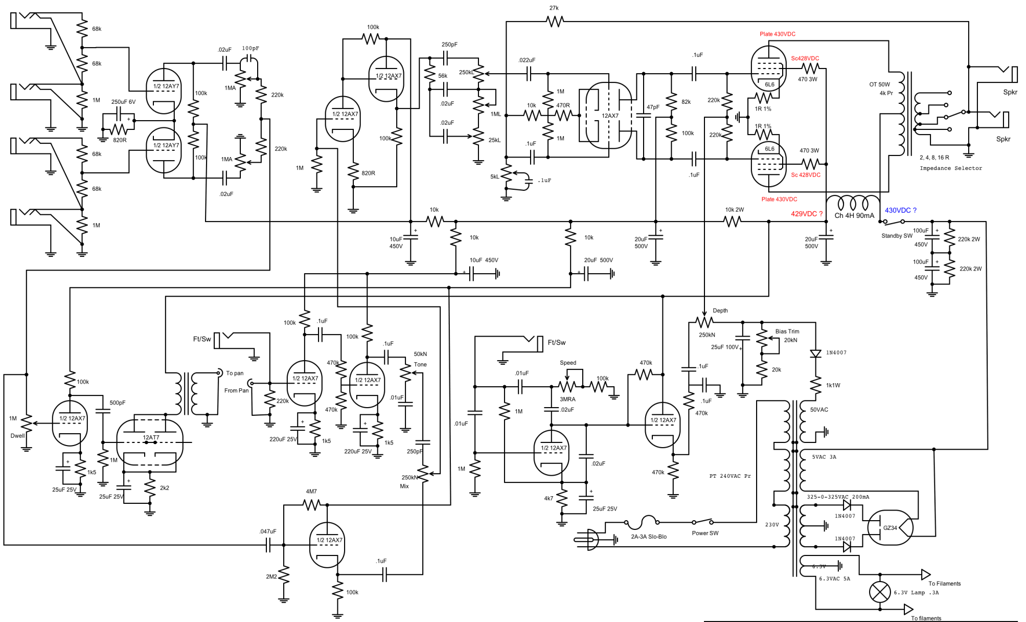
Tweed Bassman + 6G15/BF Reverb 6G16 Trem tubswell Rev 10 4/13/09 Page #
