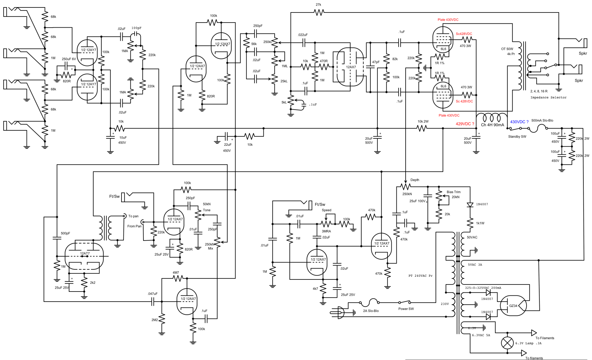
Tweed Bassman + 6G15/BF Reverb 6G16 Trem tubeswell Rev 12 5/3/09 Page #
