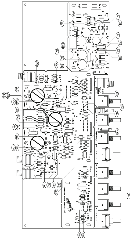
FIGURE SERVICE DIAGRAM DRAWING: 73737-003 DATE: M--JUN-07
