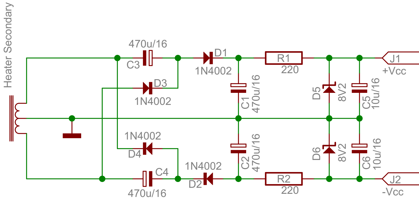
Split +/- 8V supply for opamps from center tapped heater secondary
