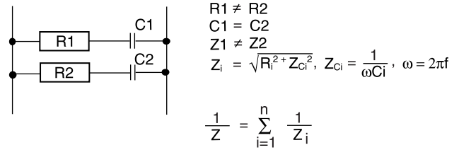
Fig. 2 - Detail from an equivalent circuit diagram for two surface elements
