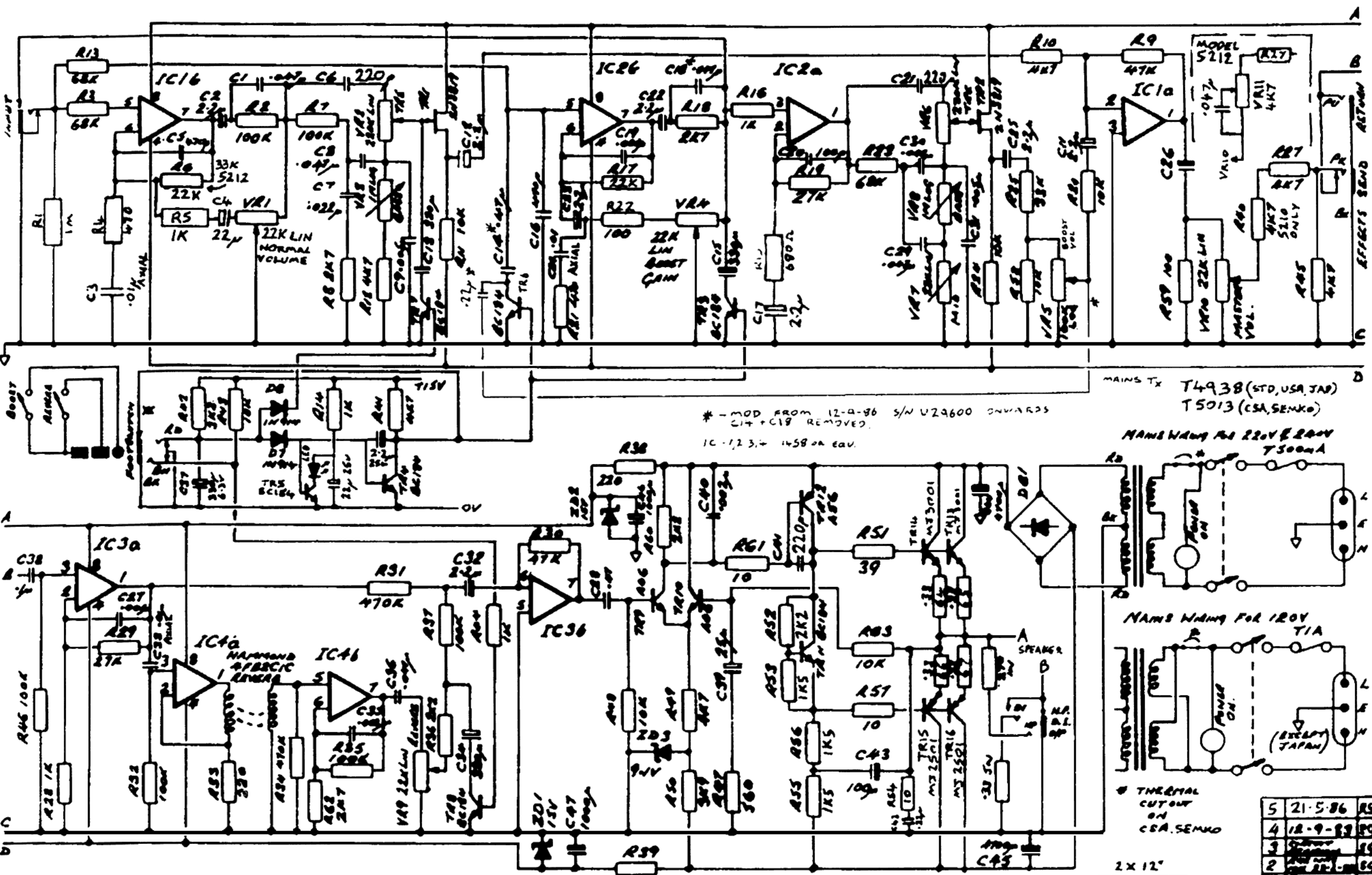
5210 MODEL 5212 50Watt Transistor Reverb Combo — CIRCUIT DIAGRAM
