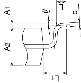
Detail F
