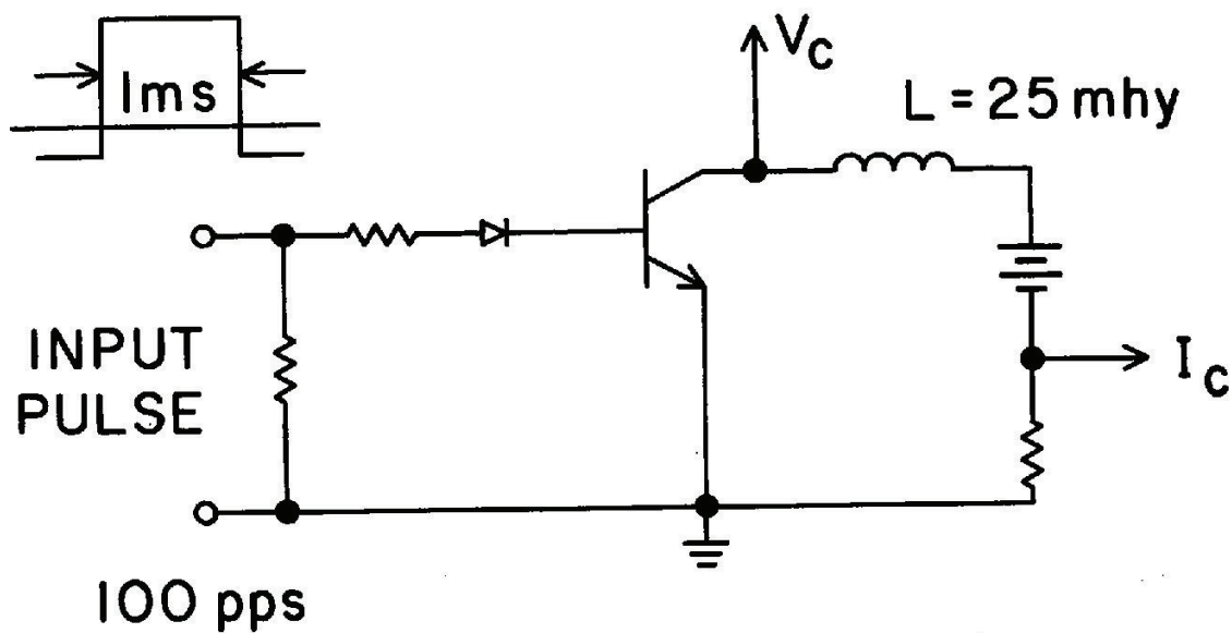
Figure 1 Second breakdown test circuit
