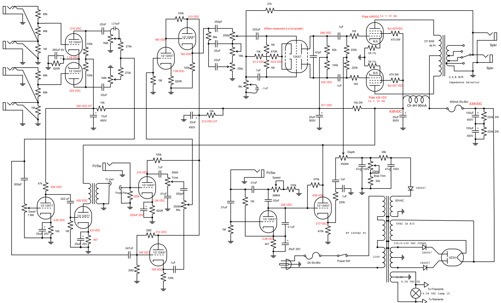
Tweed Bassman + 6G15/BF Reverb 6G16 Trem tubeswell Rev 12 g 8/12/09 Page #
