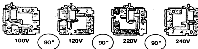
Figure 2.2 - Voltage Selector Card Orientation
