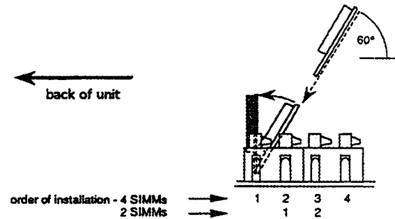
Figure 2.7 - SIMM installation
