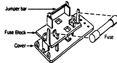
Figure 2.3 - American fuse
