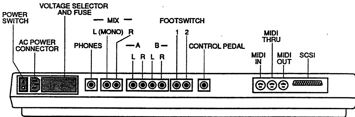
Figure 2.8 - Rear Panel Connection Layout
