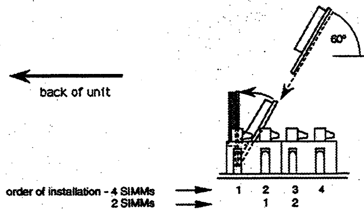
Figure 2.12 - SIMM Installation
