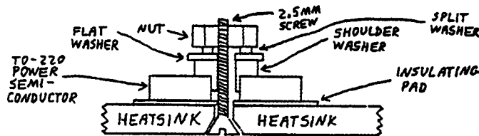
Figure 5.1.2.1 - Heatsink mounting detail
