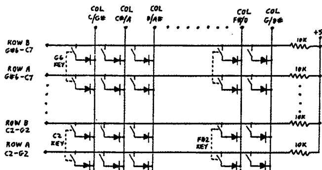
Figure 5.1.1.1 - Portion of keyswitch matrix
