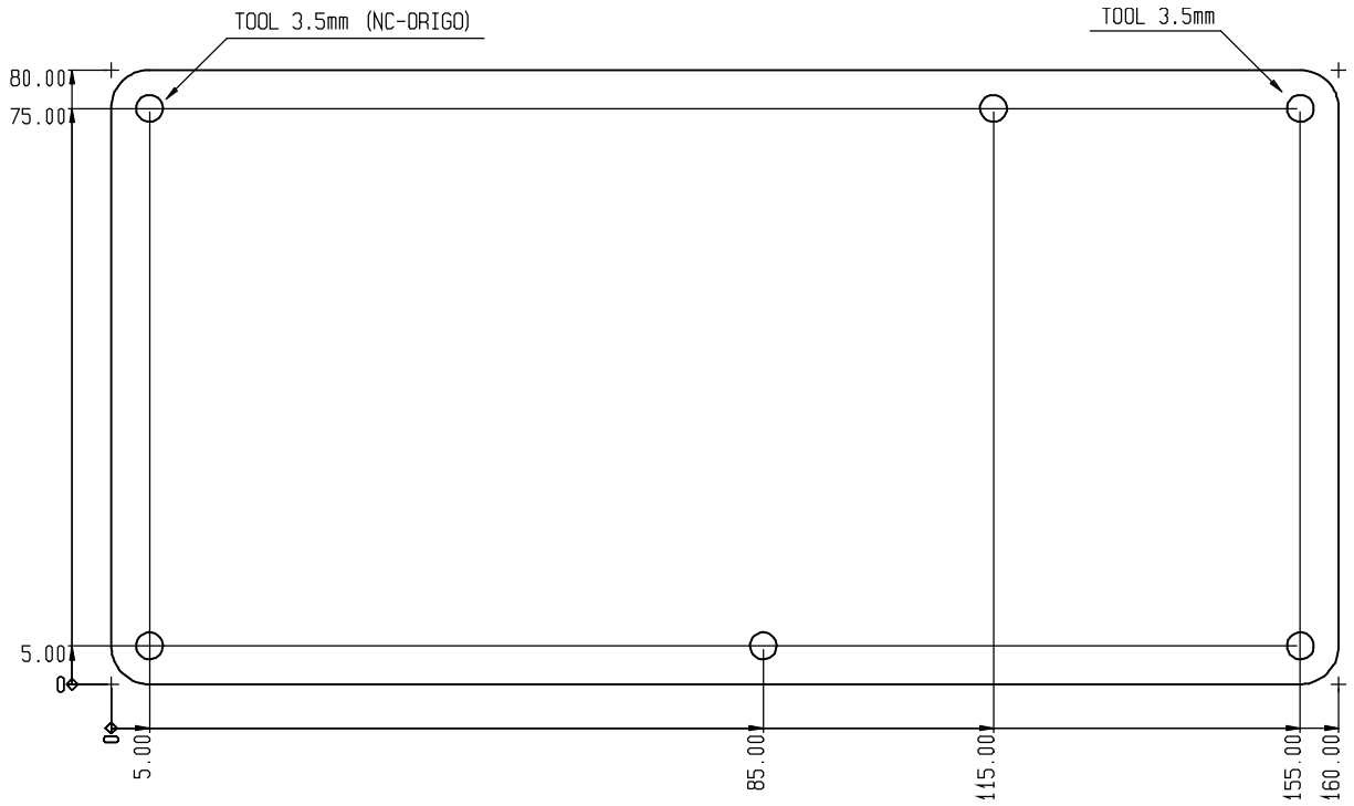
Figure 22: PCB drill pattern.
