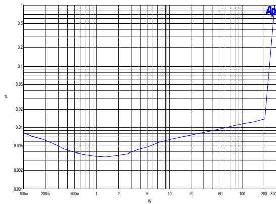
TIM vs. output power. R_L = 4\Omega , \text{TIM}@10\text{W} = 0.006\%
