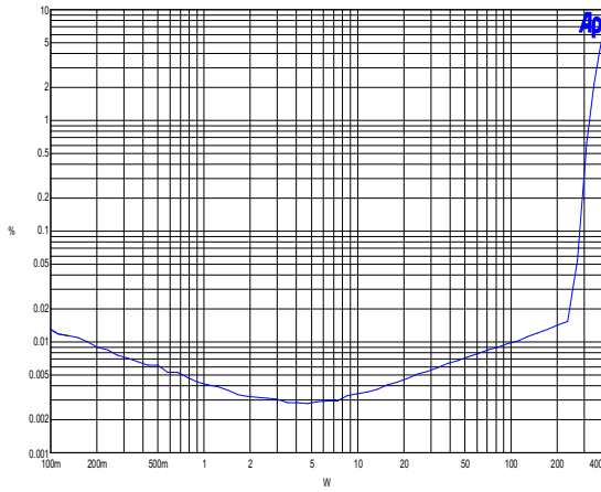
TIM vs. output power. R_L = 4\Omega , TIM@10W = 0.004%
