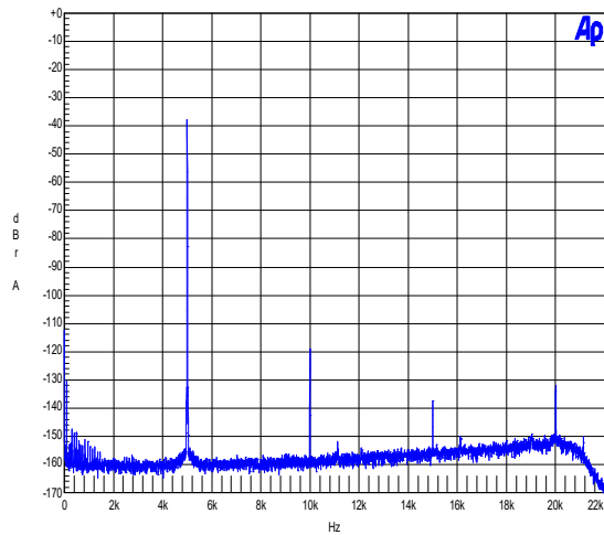
f = 5kHz. Po = 100mW. 4Ω loading. (Relative to 125W into 4 ohm)
