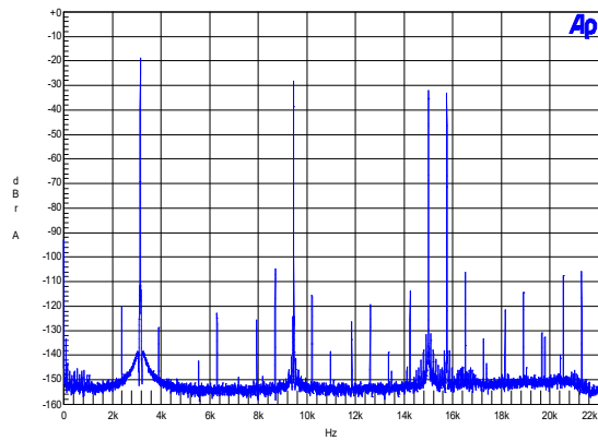
TIM FFT analysis. R_L = 4\Omega , P_o = 10\text{W} .
