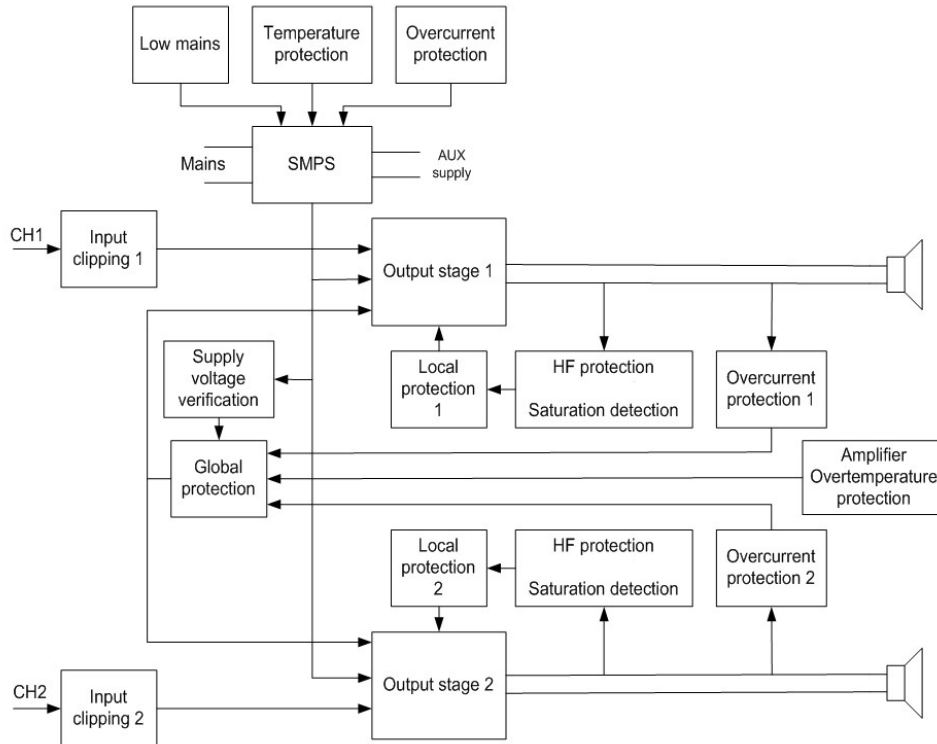
Figure 15: Protection schematic
