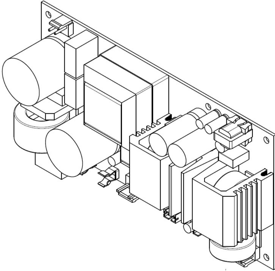
Figure 21: 3D-view of the ICEpower125ASX2 board.
