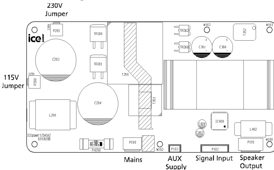
Figure 2: ICEpower125ASX2 connections
