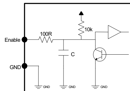
Figure 12: Enable pin interface.
