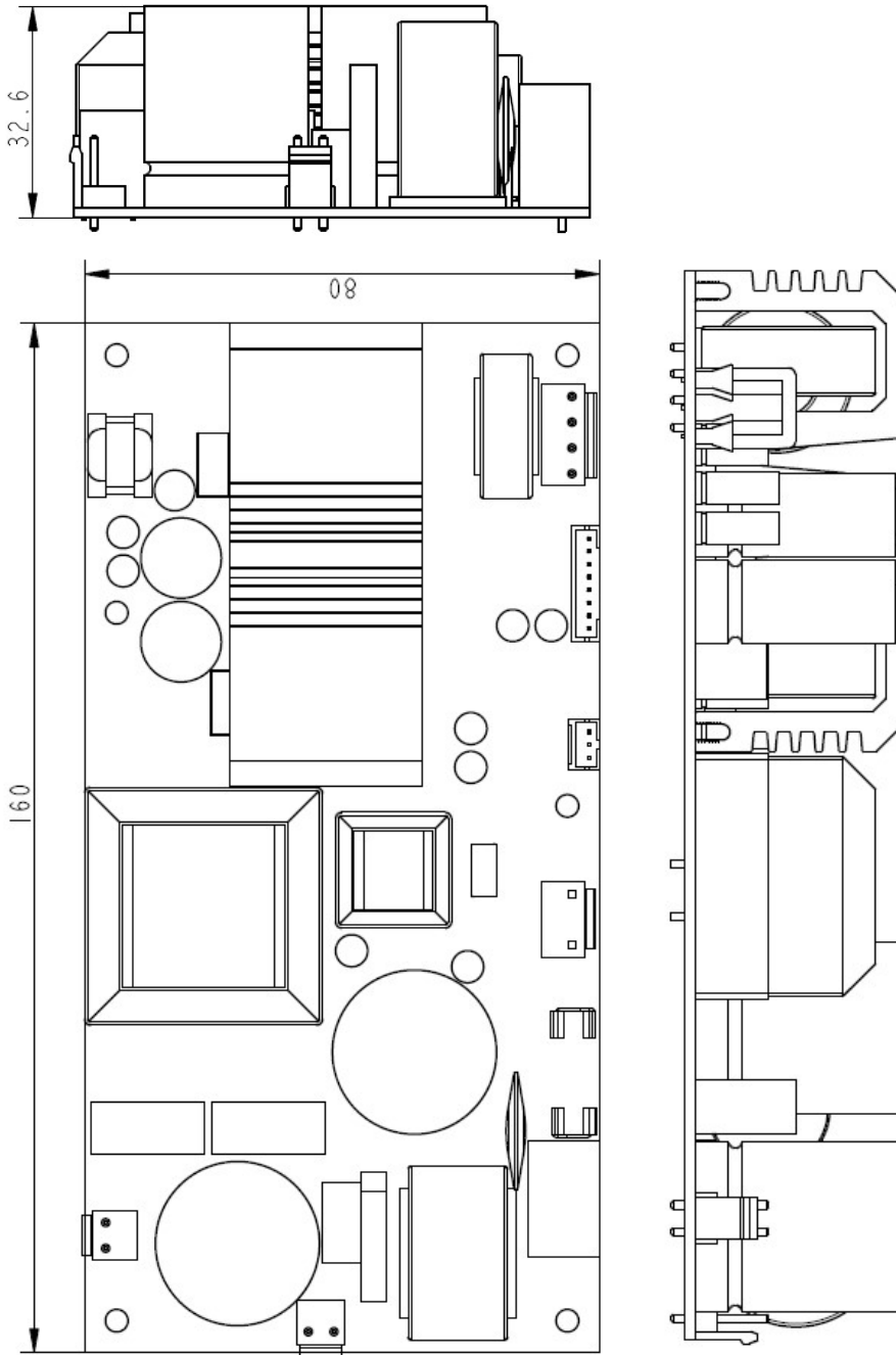
Figure 20: Physical dimensions in mm.
