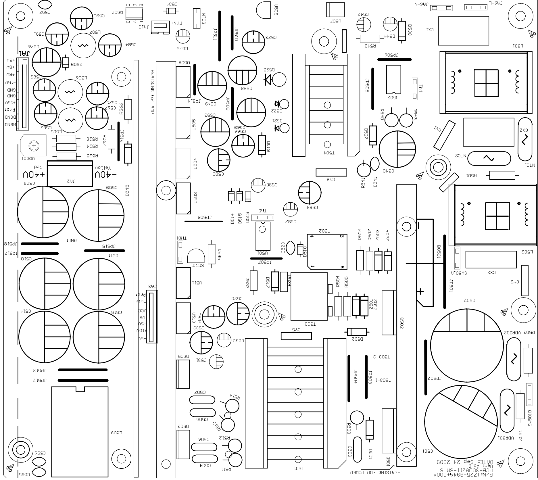
SMPS PCB top side
