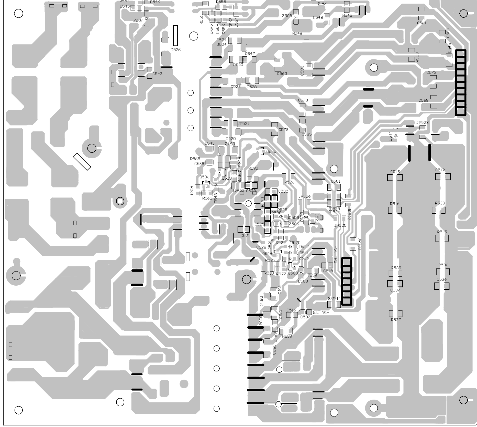
SMPS PCB bottom side
