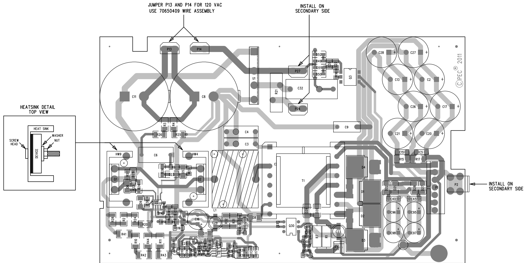
PVXp POWER SUPPLY - PRIMARY and SECONDARY SIDE VIEW
