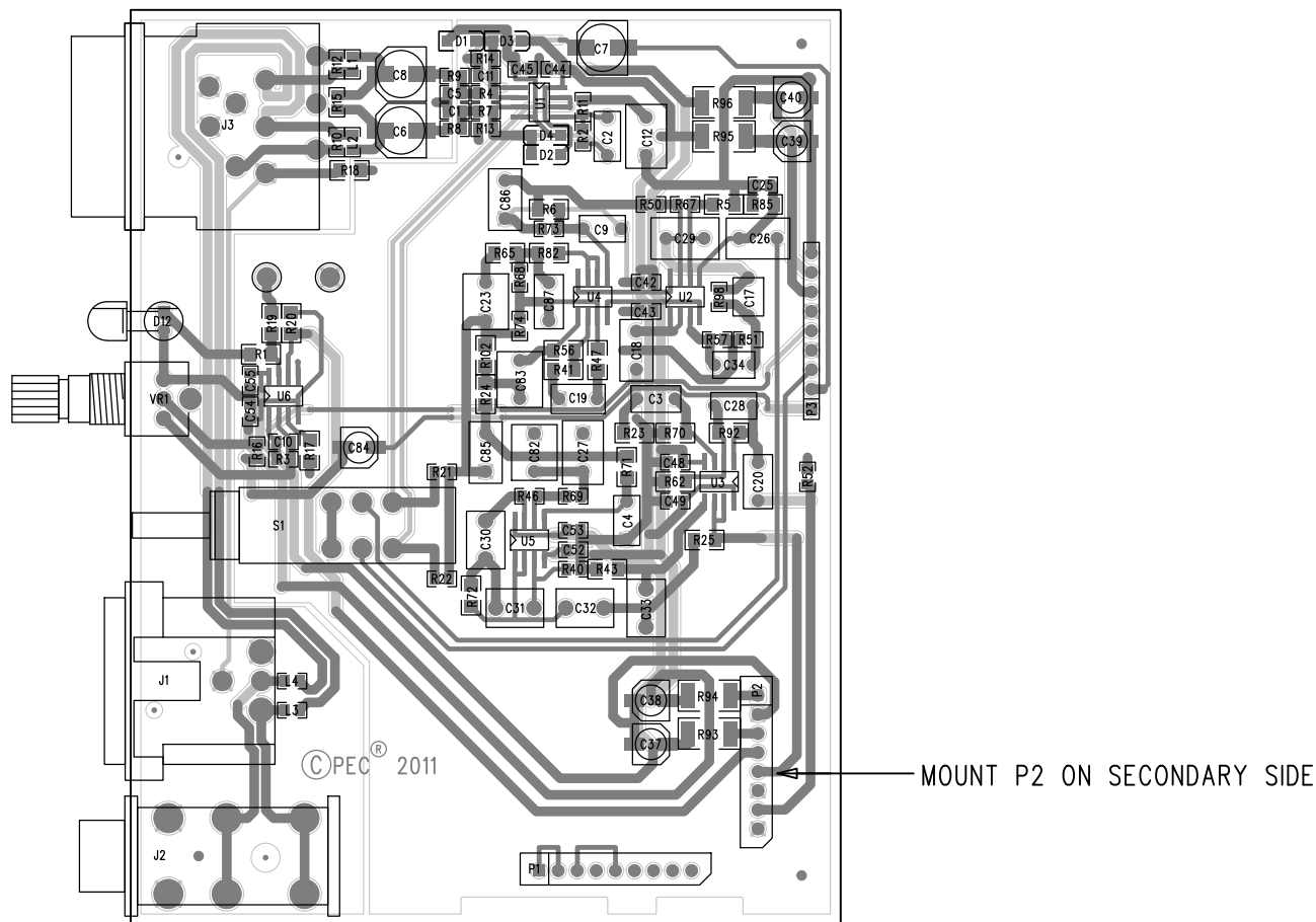
PVXp Preamp - Primary Side View
