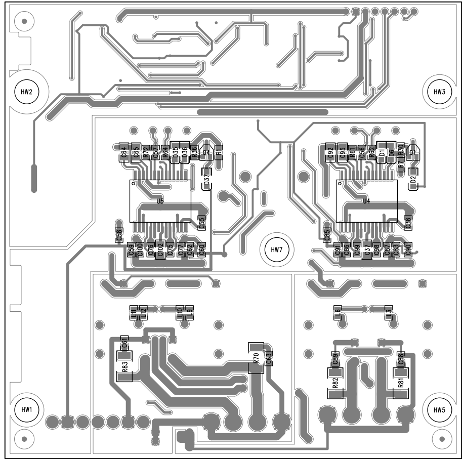
PVXp Power Amp - Secondary Side View
