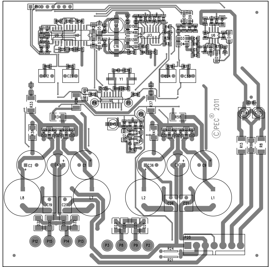
PVXp Power Amp - Primary Side View
